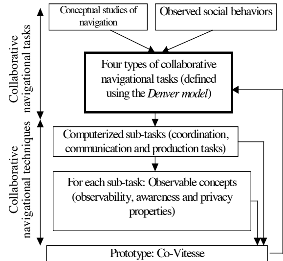
Figure 1: Design method.
