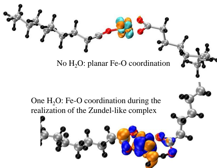
Figure II-21. Fe-based steirates: Spin density distribution at 10^{-3} e/\text{\AA}^3
