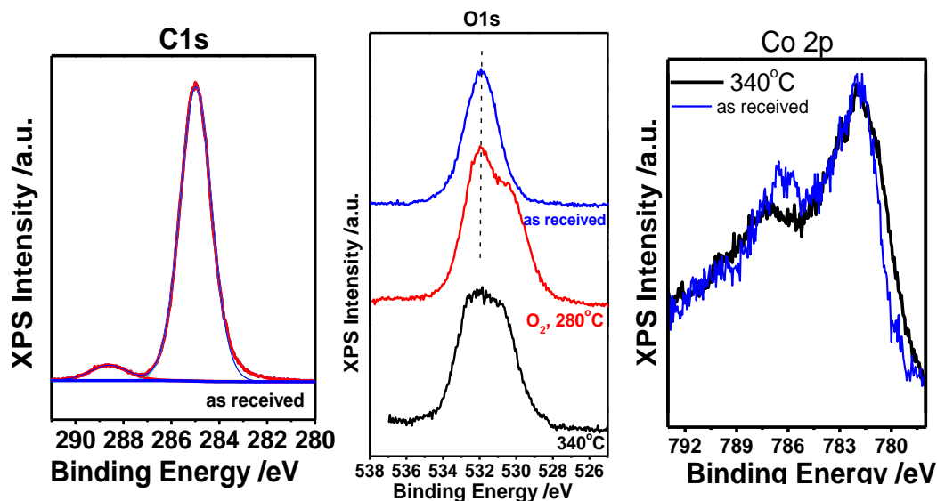
Figure II-16. C 1s, O 1s and Co 2p XPS spectra of the as-received Co-stearate and after annealing
