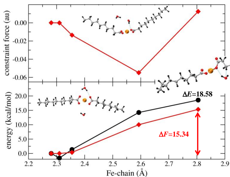
Figure II.24. Fe-based stearates at 300 K in wet conditions. Constraint force (upper panel) and free and total energies (lower panel) for the desorption of the Fe-based stearates at 300 K in wet conditions. The free energy profile is shown by the red line and the total energy one by the black line. The free energy barrier to the desorption, indicated in the lower panel, is already larger than 15.34 kcal/mol (calculations still in progress) before the completion of the desorption process.
