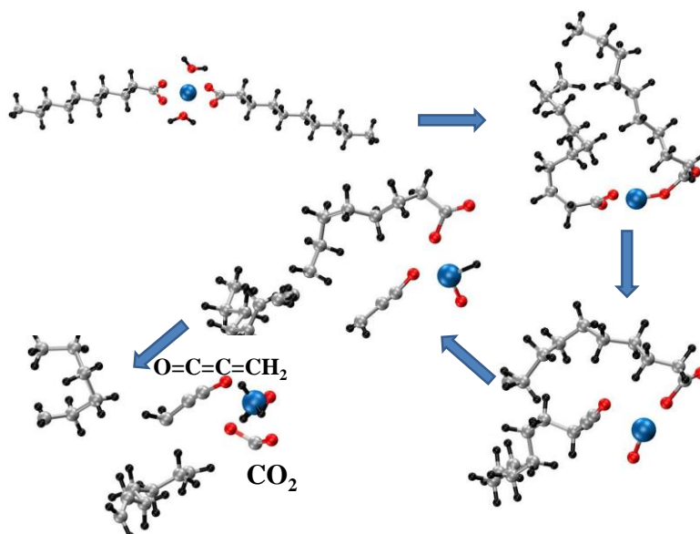
Figure II.27. Co-based steirates at 300 K in wet conditions
