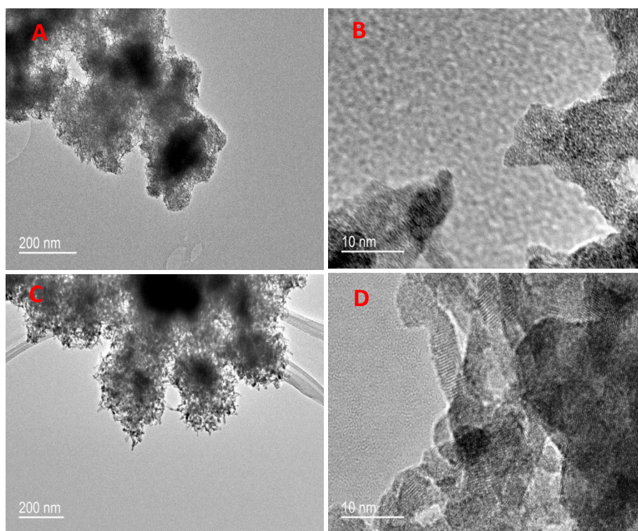
Figure V-9. TEM images of Nb 2 O 5 before (A and B) and after (C and D) calcination.
