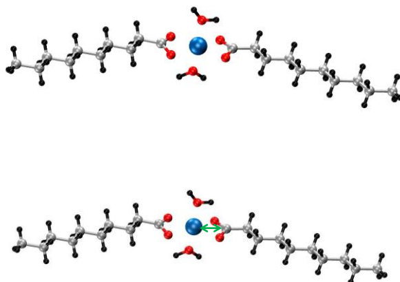
Figure II.25. Co-based stearates at 300 K in wet conditions. The green arrow indicates the reaction coordinate used in Blue Moon ensemble simulations to desorb the stearate chain.
