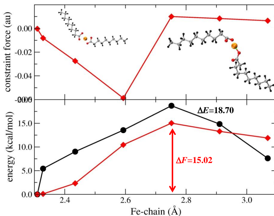
Figure II-23. Equilibrium geometries of Fe-based stearates at 300 K in wet conditions. Constraint force (upper panel) and free and total energies (lower panel) for the desorption of the chain in Fe-based stearates at 300 K in dry conditions. The free energy profile is shown by the red line and the total energy one by the black line. The free energy barrier to the desorption, indicated in the lower panel, amounts to 15.02 kcal/mol.
