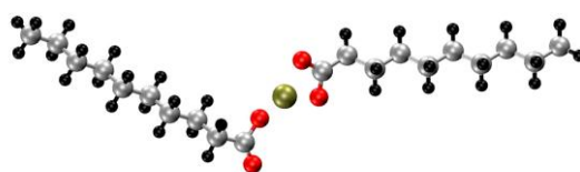
Figure II-18. Equilibrium geometries of Fe stearates at 300 K (dry) in the absence of water.
