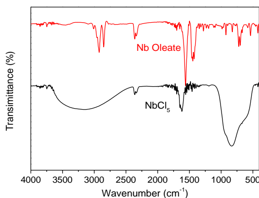
Figure V-2. IR spectra of \text{NbCl}_5 and obtained Nb Oleate.
