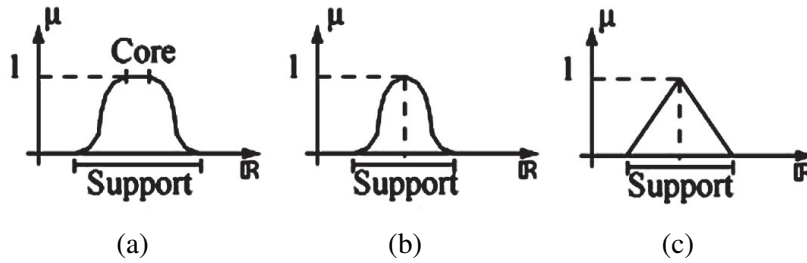
Fig. 9. Membership functions of fuzzy quantities: (a) fuzzy interval, (b) fuzzy number, (c) triangular fuzzy number
