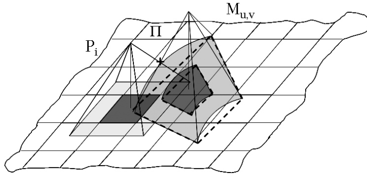
Fig. 14. Computation of \Pi(P_i, M_{u,v}) as intersection height of P_i et M_{u,v} . The dotted lines represent the approximation of the mask element.
