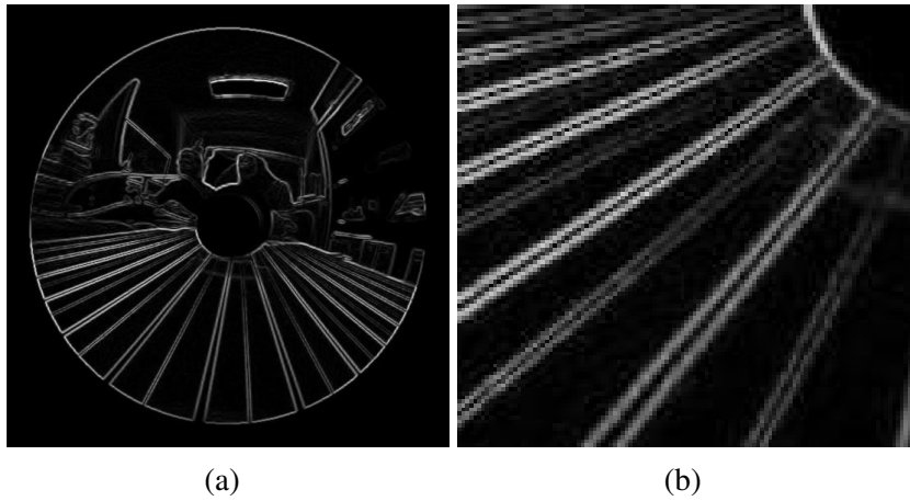
Fig. 26. (a) Deriche filter applied on the omnidirectional image and (b) Zoom
