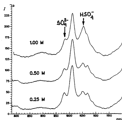
Figure 3: Raman spectra of the ARA membrane immersed in \text{H}_2\text{SO}_4 aqueous solution of increasing molar concentration.
