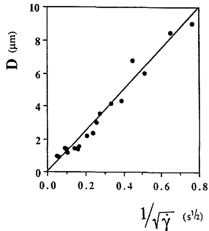
Fig. 3. — Measurements of the characteristic size (diameter D ) of the spherulites obtained with the AOT/brine sample as a function of the inverse of the square root of the shear rate (see Eq. (3) in the text).
