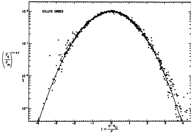
FIG. 2. — Plot of the values (F_q/F_m)^{1+\epsilon t} versus t for 58 experimental distributions for heavy ions ( Z \geq 16 ) in dilute gas strippers. The curve corresponds to the asymmetric distribution F_q/F_m = \exp\{-0.5 t^2/(1 + \epsilon t)\} .
