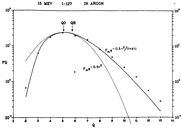
FIG. 1. — Plot of charge state intensities in % versus q for 15 MeV ^{127}\text{I} in Ar. The solid line is a least squares fit to the experimental values (Ref. [3]) with F_m = 23.3 , q_0 = 5.07 , \rho = 1.67 , \epsilon = 0.31 , and t = (q - q_0)/\rho . The dashed line corresponds to \epsilon = 0 , i.e. a pure Gaussian.
