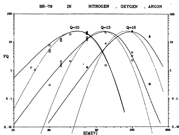
FIG. 7. — Charge state intensities versus energy for ^{79}\text{Br} in \text{N}_2 , \text{O}_2 , and Ar. The squares, circles, and triangles correspond to q = 10, 13 , and 16 , respectively. The solid and dashed curves are predictions with asymmetric and Gaussian distributions, respectively.
