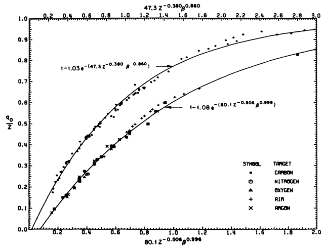
FIG. 3. — Plot of q_0/Z versus reduced velocity functions for heavy ions ( Z \geq 16 ) in carbon (upper abscissa) and dilute gas (lower abscissa) strippers. The curves represent least squares fits using the formula q_0/Z = 1 - k \cdot \exp\{-AZ^{\alpha}\beta^{\gamma}\} .
