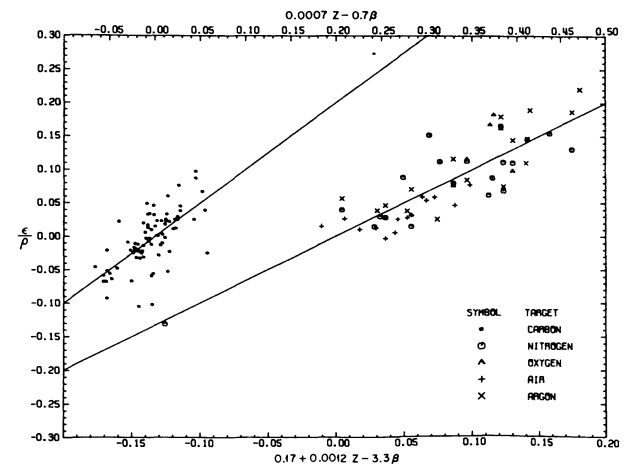
FIG. 5. — Plot of \epsilon/\rho versus functions of the form A + B.Z + C.\beta for carbon (upper abscissa) and dilute gas (lower abscissa) strippers. The curves represent least squares fits.
