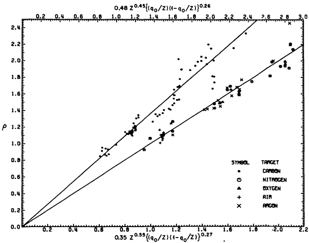
FIG. 4. — Plot of \rho versus functions of the form AZ^{\alpha} \{ (q_0/Z) (1 - q_0/Z) \}^{\gamma} for carbon (upper abscissa) and dilute gas (lower abscissa) strippers. The curves represent least squares fits.
