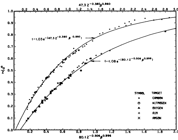
FIG. 3. — Plot of q_0/Z versus reduced velocity functions for heavy ions ( Z \geq 16 ) in carbon (upper abscissa) and dilute gas (lower abscissa) strippers. The curves represent least squares fits using the formula q_0/Z = 1 - k \cdot \exp \{ -AZ^{\alpha} \beta^{\gamma} \} .
