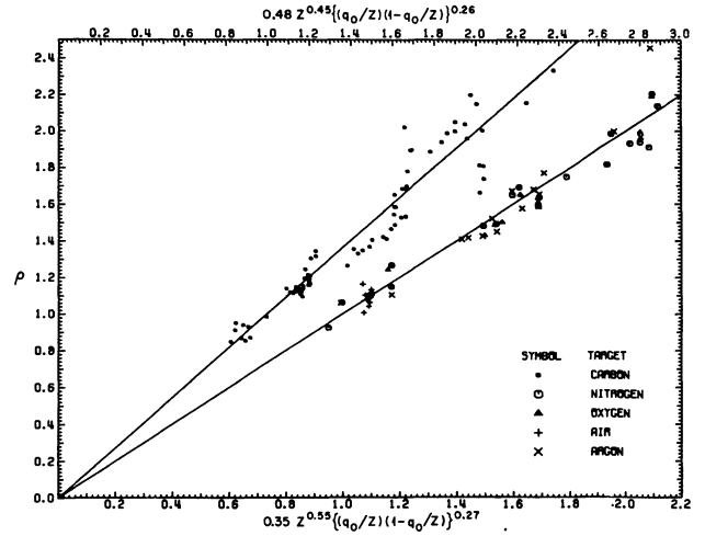
FIG. 4. — Plot of \rho versus functions of the form AZ^{\alpha}\{(q_0/Z)/(1 - q_0/Z)\}^{\gamma} for carbon (upper abscissa) and dilute gas (lower abscissa) strippers. The curves represent least squares fits.
