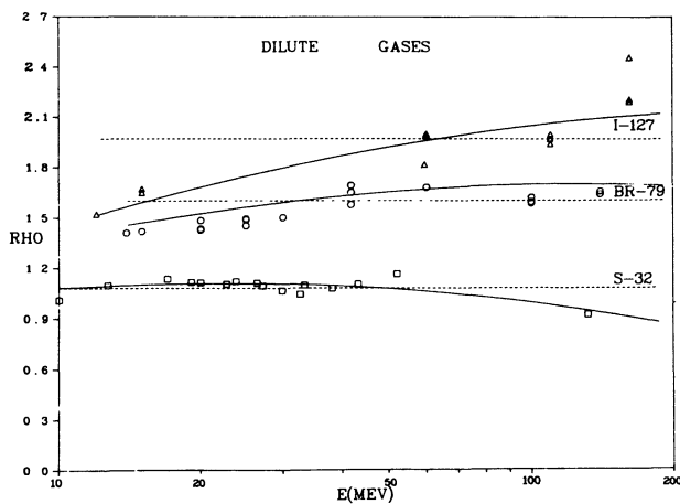
FIG. 6. — Plot of \rho versus energy for ^{32}\text{S} ions (squares), ^{79}\text{Br} ions (circles), and ^{127}\text{I} ions (triangles) in dilute gases. The dashed curves correspond to \rho = 0.27 \sqrt{Z} , and the solid curves to \rho = 0.35 Z^{0.55} \{ (q_0/Z) (1 - q_0/Z) \}^{0.27} .
