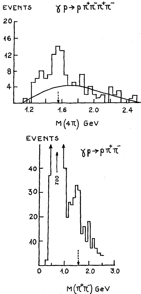
FIG. 2. — a) 4\pi mass distribution in the reaction
