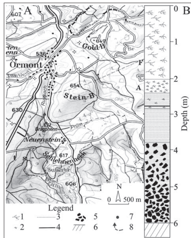
Fig. 6: The Bragphenn site (A) and the lithostratigraphical column at the thickest place of the deposits (B).
