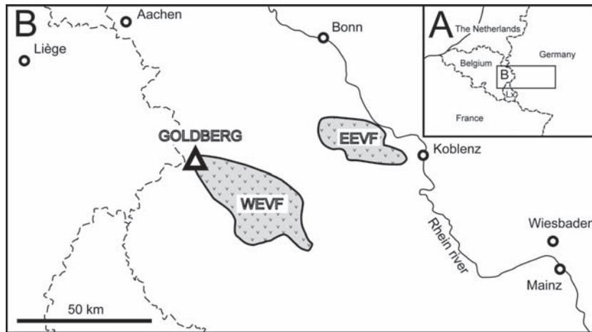
Fig. 1: Location of the Goldberg volcano, as well as the West and East Eifel volcanic fields respectively.
