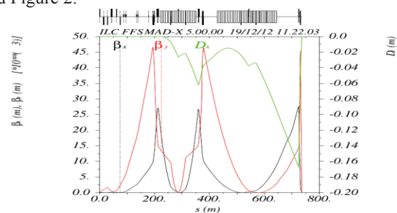
Figure 2: The linear lattice functions of ILC FFS with \beta_x^*/\beta_y^*=15\text{mm}/0.4\text{mm} .
