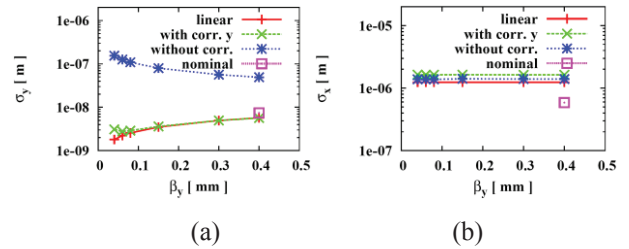
Figure 6: (a) The vertical beam size as a function of \beta y^* when \beta x^*=75\text{mm} . (b) The impact of the variable \beta y^* on \sigma x^* when \beta x^*=75\text{mm} .
