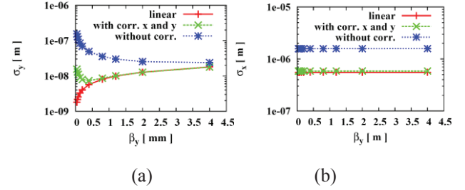
Figure 4: (a) The vertical beam size \sigma y^* as a function of \beta y^* when \beta x^*=15\text{mm} . (b) The impact of the variable \beta y^* on \sigma x^* when \beta x^*=15\text{mm} .
