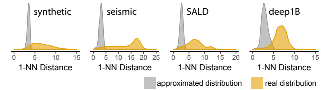
Fig. 10: Real distribution of 1-NN distances and its query-agnostic approximation based on Ciaccia and Patella [32]. All datasets contain 100K series.
