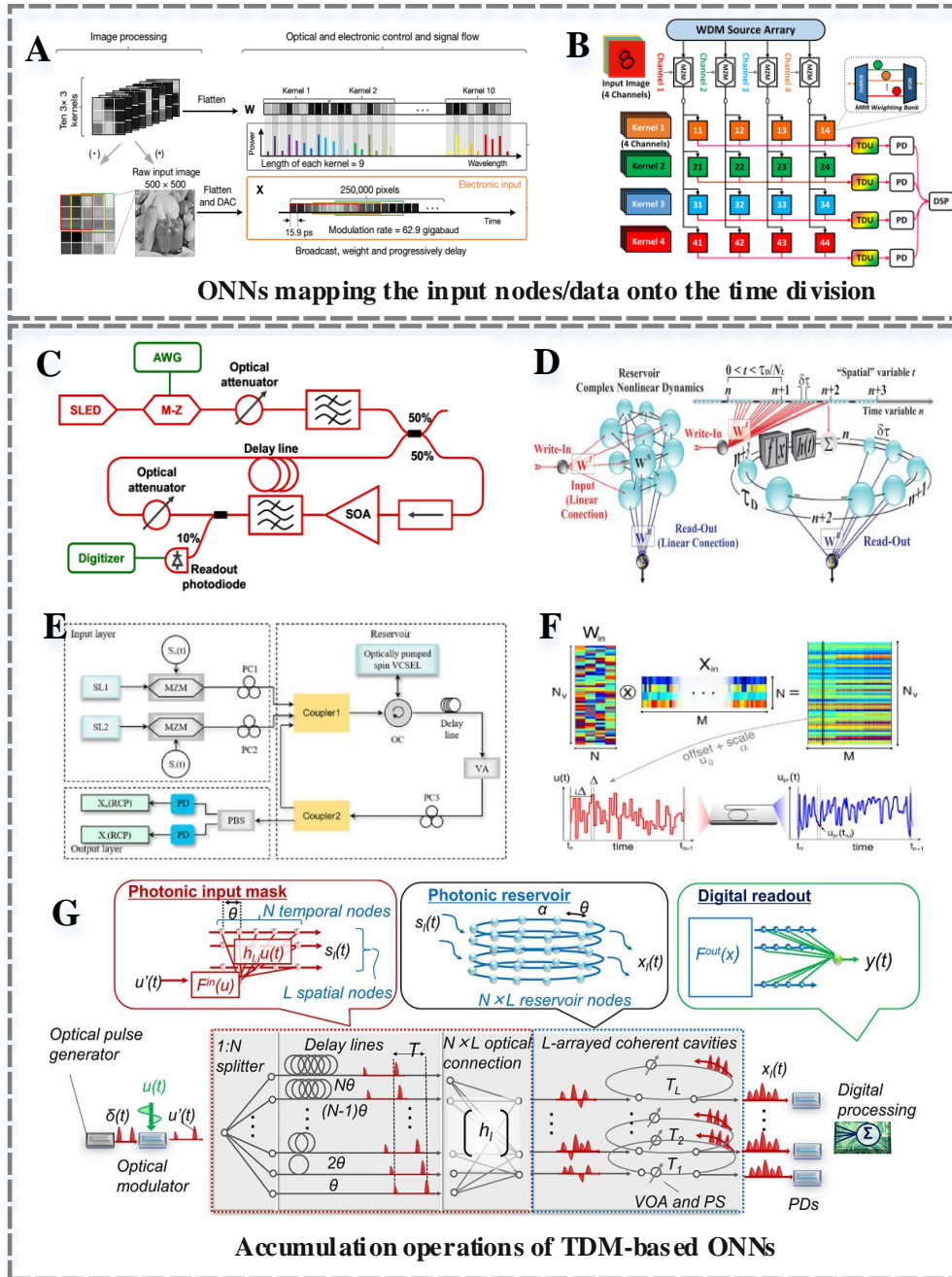
Fig. 5 Advances in TDM-based ONNs. (A, B) ONNs exploiting TDM to implement large-scale fan-in/-out [39], [110]. (C) Time-delay reservoir computing (TD-RC) based on SOA [119]. (D) TD-RC based on electro-optic phase-delay oscillator [121]. (E) TD-RC based on an optically pumped spin VCSEL [123]. (F) TD-RC based on a silicon microring [124]. (G) Scalable RC on coherent linear photonic processor [133].
