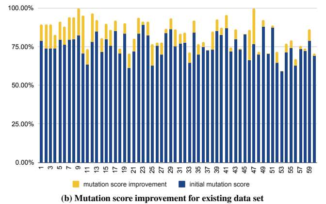
Figure 8: Mutation score improvement by test amplification
