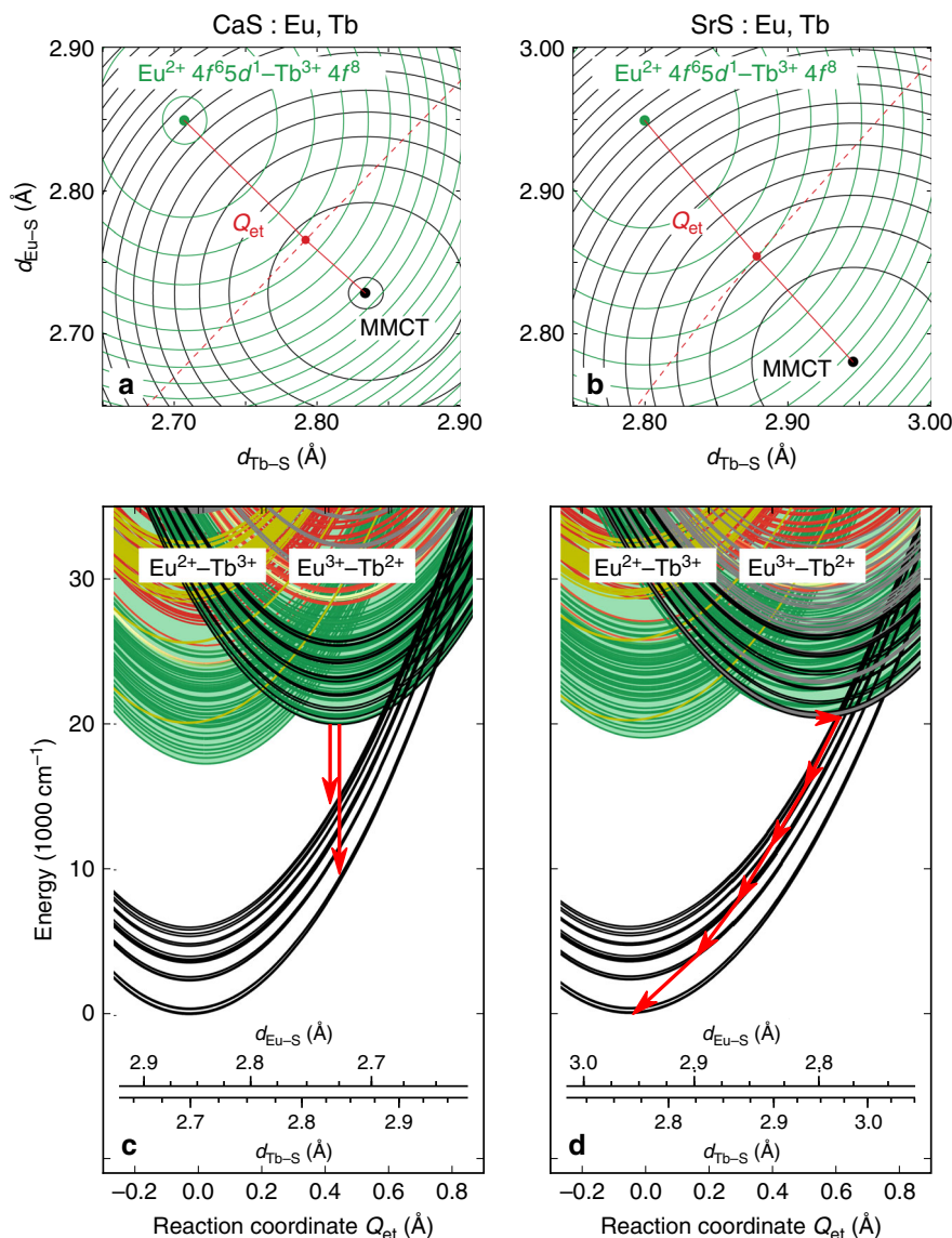
Fig. 6 Metal-to-metal charge transfer many-electron diagrams. Contour plots of selected potential energy surfaces in the two-dimensional configurational space ( d_{\text{Eu-S}} , d_{\text{Tb-S}} ) ( a , b ) and configurational coordinate diagrams along the electron transfer reaction coordinate ( Q_{\text{et}} ) ( c , d ) for Eu-Tb pairs in CaS ( a , c ) and SrS ( b , d ). The configurational coordinate diagrams display the following levels for the \text{Eu}^{2+}\text{-Tb}^{3+} configuration: 4f^7(^8S)\text{-}4f^8(^7F) (black), 4f^65d^1_{2g} - 4f^8(1A_{1g}) (green for high-spin states, red for low-spin states) and 4f^7(^8S)\text{-}4f^8(^5D, L, G) (gold), and following levels for the \text{Eu}^{3+}\text{-Tb}^{2+} configuration: 4f^6(^7F)\text{-}4f^85d^1(1\Gamma_{7g}) (black), 4f^6(1A_{1g})\text{-}4f^85d^1_{2g} (green for high-spin states, red for low-spin states), and 4f^6(1A_{1g})\text{-}4f^9 (gray). The quasi-continuum formed by all other levels of the Eu-Tb pair, where none of both ions is in its ground state are represented by the green-colored background. The contour plots display the isolines corresponding to the \text{Eu}^{2+}4f^65d^1(1\Gamma_{8g})\text{-Tb}^{3+}4f^8(1A_{1g}) and \text{Eu}^{3+}4f^6(^7F)\text{-Tb}^{2+}4f^85d^1(1\Gamma_{7g}) (lowest metal-to-metal charge transfer (MMCT) state) surfaces. The reaction coordinate is indicated in red, along with the intersection between both surfaces (dashed red line).
