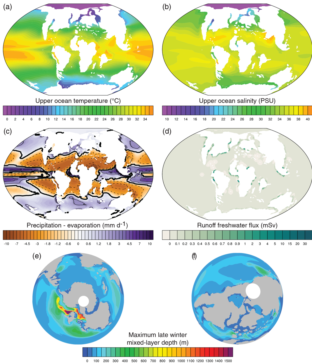
Figure 8. Climate diagnostics for the Maastrichtian simulation. (a) Surface ocean (upper 100 m) temperature (°C). (b) Surface ocean (upper 100 m) salinity (PSU). (c) Precipitation minus evaporation (mm d -1 ). (d) Runoff freshwater flux (mSv). (e, f) Late winter maximal mixed layer depth (m).
