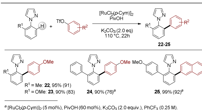
Scheme 4 Synthesis of unequally o -difunctionalized azoles.
