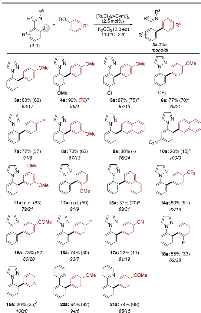
a PhCF 3 (0.25 M). b 2-naphthyl triflate (1.5 equiv.), [RuCl 2 ( p -Cym)] 2 (5 mol%), PivOH (60 mol%), K 2 CO 3 (2.0 equiv.), PhCF 3 (0.25 M). c 1 (1.0 equiv.), 3-pyridine triflate (3.0 equiv.), [RuCl 2 ( p -Cym)] 2 (2.5 mol%), PivOH (30 mol%), K 2 CO 3 (4.0 equiv.), PhCF 3 (0.25 M).
