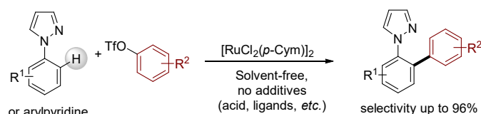
Scheme 1 Synthetic selective access to o -monoarylated azoles or pyridines under solvent- and additives-free conditions.
