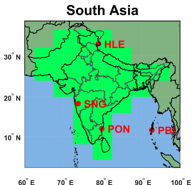
Figure 1. The South Asia region boundaries (light green) used to aggregate CO 2 fluxes. The locations of the four flask CO 2 measurement stations (Port Blair [PBL], Pondicherry [PON], Sinhad [SNG], and Hanle [HLE]) are overlaid (red dots) for reference.
