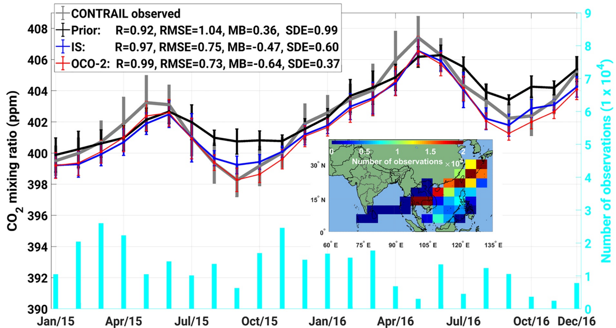
Figure 6. Comparison of monthly averaged CONTRAIL observed \text{CO}_2 mixing ratio (ppm) at the altitude range of ~5 to 13 km near and downwind of the South Asia region (see map in the inset) and the values simulated from the prior model and those optimized with in situ (IS) and OCO-2 (LN + LG assimilation) observations. Error bars represent the standard deviation of mean monthly values. The legend contains evaluation statistics of monthly mean values during 2015–2016 and the inset shows the total number of CONTRAIL observations per grid cell. The cyan bars represent total number of CONTRAIL observations per month.
