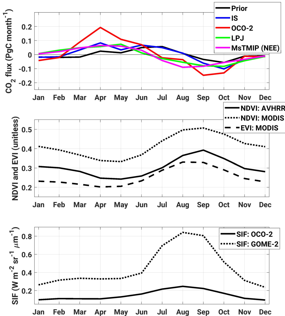
Figure 4. Comparison of South Asian multi-year mean monthly NBE (PgC month -1 ) from the prior model (CASA; solid black line), posteriors optimized with IS (blue) and OCO-2 LN + LG (red) observations, NBE from the LPJ model (green), and the MsTMIP ensemble mean NEE (“optimal” or “weighted” ensemble mean from 15 global land surface models; magenta; top row). These values are further compared with NDVI (unitless) from the AVHRR and MODIS, EVI (unitless) from MODIS (middle row), and SIF (W m -2 sr -1 μm -1 ) from the GOME-2 and OCO-2 (bottom row).
