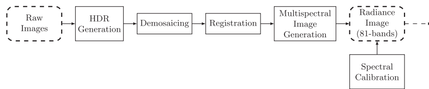
FIGURE 1 | Data acquisition pipeline. Raw images are captured using a CPFA camera with four polarization angles, in front of spectral bandpass filters as described in Section 2.1 . Pre-processing steps (HDR, demosaicing, and registration) are described in Section 2.1 , whereas spectral image reconstruction is described in Section 2.2 . The dotted arrow corresponds to the connection toward Figure 3 .
