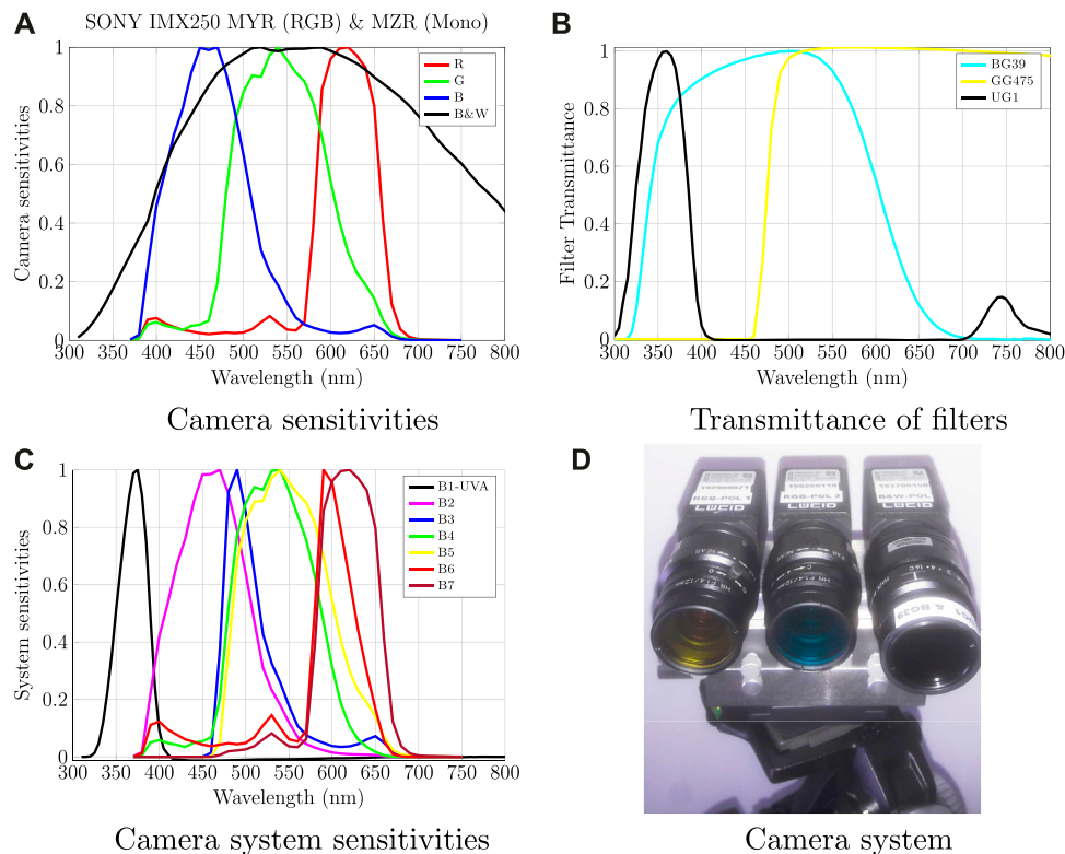
FIGURE 2 | (A) Normalized spectral sensitivities of the two cameras used. (B) Transmittance of the bandpass filters. (C) Total system sensitivity, which is a combination of the camera sensitivities with the bandpass filters. We show only spectral sensitivities for the 0^\circ polarization channels as spectral sensitivities of all polarization channels are very similar.
