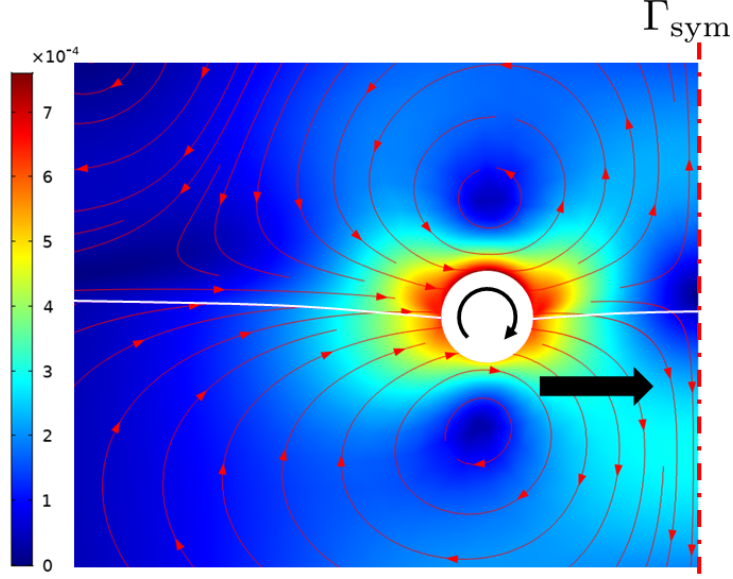
Figure 3: Snapshot of the velocity field for rotating particles undergoing a capillary attraction (time t^* = 5.6 \times 10^4 ; final time at contact: t^* = 5.85 \times 10^4 ). Only the left half of the computational domain is considered due to the symmetry axis \Gamma_{\text{sym}} (see Fig. 1a). The particle translates to the right whilst rotating clockwise (curved black arrow). The streamlines are represented by red arrow lines whereas the solid white line indicates the fluid interface ( \phi = 0 ). The color bar gives the scaled velocity amplitude ( |\mathbf{v}|/U_{\text{cap}} , see Sec. 2). Parameters: \mu^* = 0.05 , \theta = 100^\circ , Cn = 0.04 , see also table 1.
