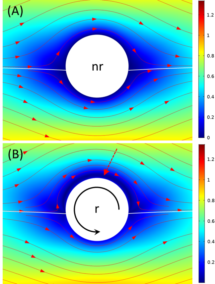
Figure 6: Steady-state streamlines in the vicinity of a non-rotating (nr) (A) and a rotating (r) (B) cylinder for problem B (Fig. 1b). The maps display the velocity magnitude scaled by the incoming flow velocity ( U_0 ) (cf. color scales). In (A), the fluid velocity is zero on the particle contour, but in (B), where the cylinder rotates counter-clockwise, the area of zero-fluid velocity is only present in the upper fluid and is shifted off the particle surface (cf. the dark blue half-circle marked by the red dashed arrow). In both cases, the solid red arrows indicate the flow streamlines while the solid white line corresponds to the fluid interface ( \phi = 0 ). Parameters: \theta = 100^\circ , \mu^* = 0.1 , Cn = 0.02 , see also table 1.
