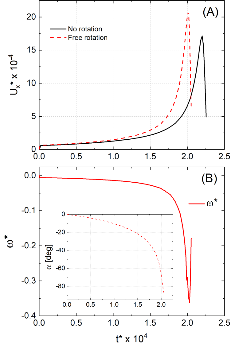
Figure 2: Results of dynamic simulations of the capillary pair interaction with and without particle rotation. (A) Particle velocity ( U_x^* = U_x/(\sigma/\mu_2) , x -component) as a function of time ( t^* = t/(\mu_2 R/\sigma) ). The particles' rotation speeds up the interaction kinetics. (B) Angular velocity ( \omega^* = \omega/(U_x^{\max}/R) ) as a function of time t^* . The inserted graph represents the time evolution of the corresponding angular displacement ( \alpha ). Parameters: \mu^* = 0.1 , \theta = 100^\circ , Cn = 0.04 , see also table 1.
