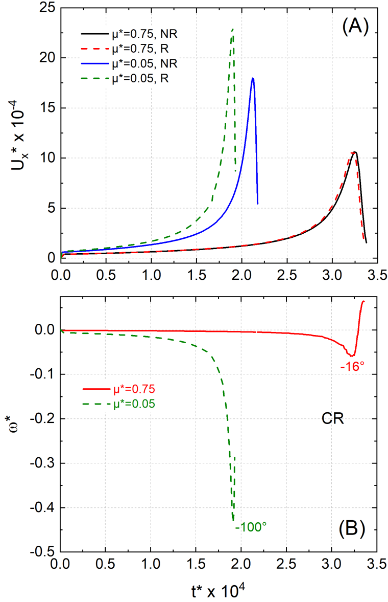
Figure 5: Influence of the viscosity ratio on the computed translational and rotational velocities of particles undergoing an attractive capillary interaction. (A) Translational velocity ( U_x^* ) and (B) Angular velocity ( \omega^* ) as a function of time ( t^* ) for two viscosity ratios. In (B), the numbers next to each curve indicate the maximum angular displacement ( \alpha ) reached at contact. NR: non-rotating; R: rotating; CR: clockwise rotation. Parameters: \theta = 100^\circ , Cn = 0.04 , see also table 1.
