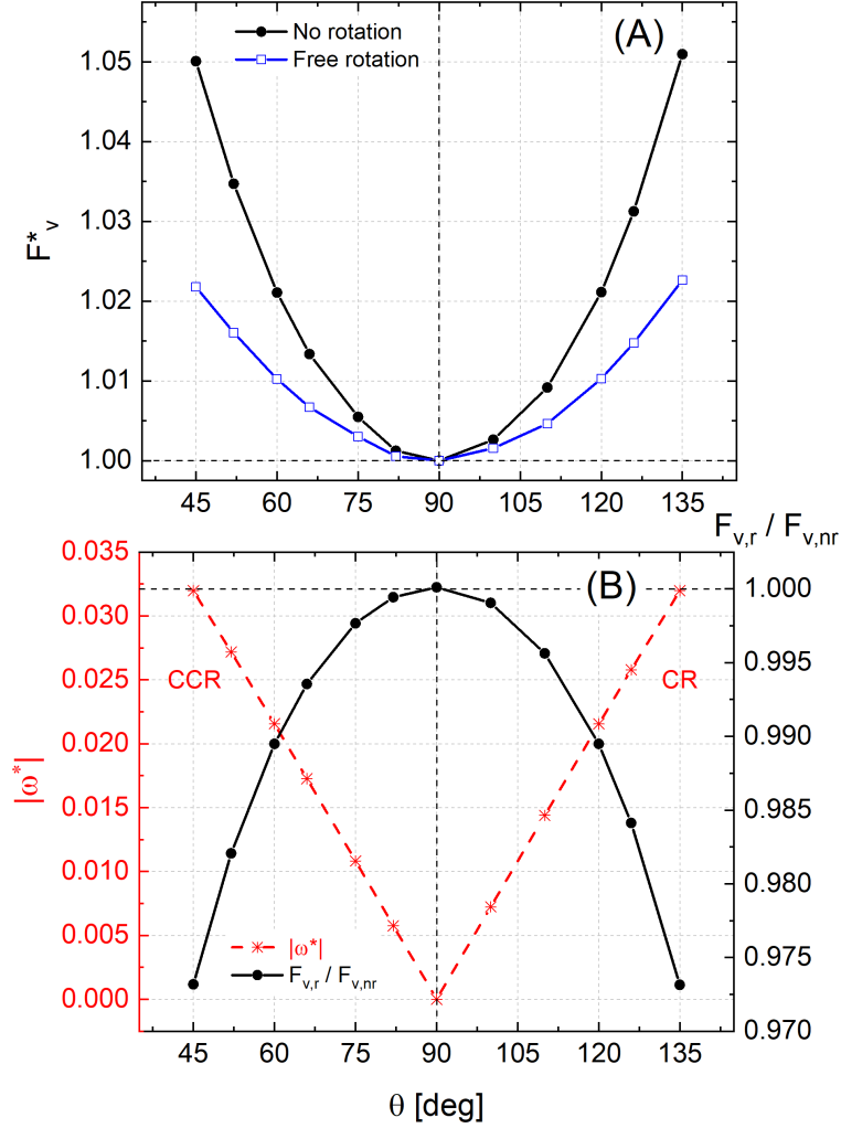
Figure 7: (A) Normalized translational drag force, F_v^* , as a function of the contact angle ( \theta ) for both rotating (r) and non-rotating (nr) particles. The normalization was done with respect to the drag force value obtained for \theta = 90^\circ in the non-rotating case. For \theta \neq 90^\circ , we see that F_{v,r}^* < F_{v,nr}^* . (B) Drag force ratio, F_{v,r}/F_{v,nr} , and absolute value of the angular velocity ( \omega^* = \omega/(U_0/R) ) as a function of \theta . It is seen that the larger |\omega^*| , the smaller the ratio F_{v,r}/F_{v,nr} compared to unity. CCR: counter-clockwise rotation ( \theta < 90^\circ ); CR: clockwise rotation ( \theta > 90^\circ ). Parameters: \mu^* = 1 , Cn = 0.02 , see also Fig. 1b and table 1.
