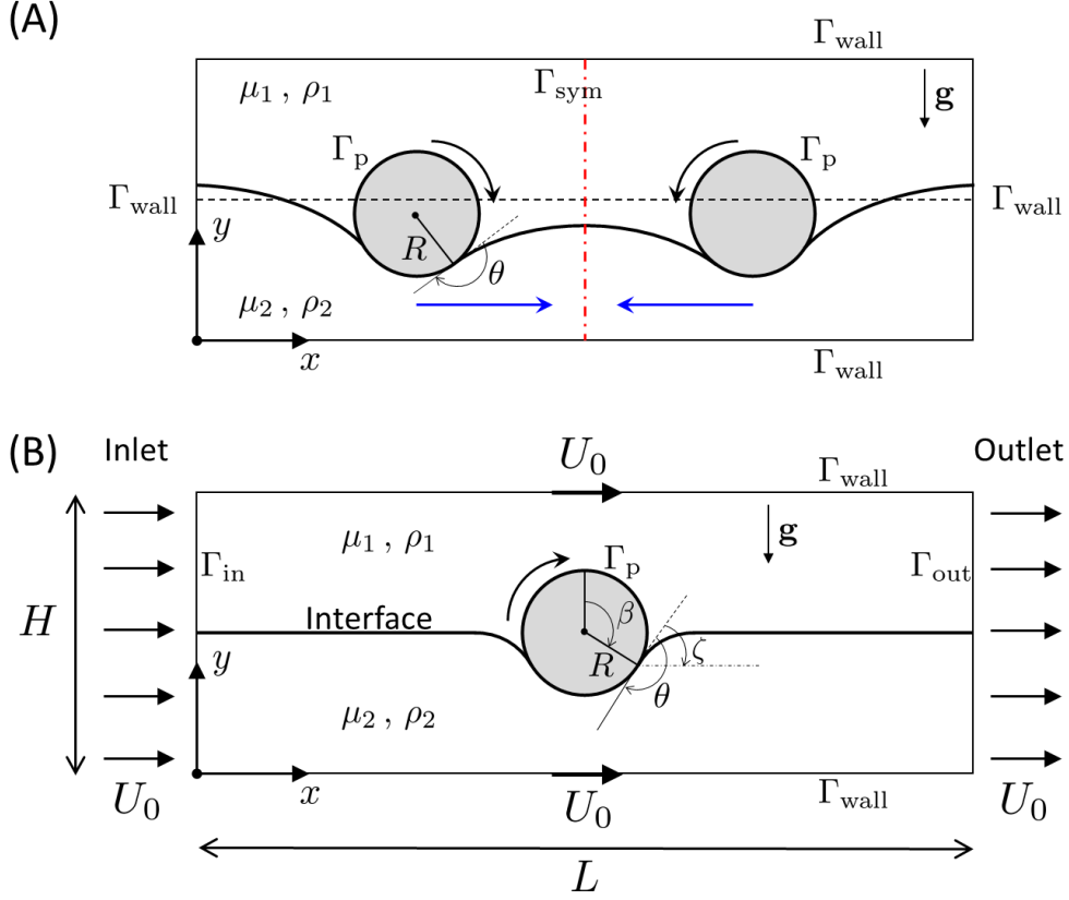
Figure 1: Two-dimensional geometries of the two problems investigated in this work. (A) Geometry for the computation of the pair capillary interaction between floating cylinders at a fluid interface (problem A). The vertical red dashed-dotted line marks the symmetry plane ( \Gamma_{\text{sym}} ) and the solid blue arrows represent the capillary attraction between the two particles due to interfacial deformations. The curved arrows indicate particle rotation. Symbols: \theta : contact angle, \mathbf{g} : gravitational acceleration. (B) Geometry for the computation of two-phase flow drag on a circular rotating cylinder confined at a fluid interface between two plane walls (problem B). Symbols: \beta : floating angle, \zeta : interface slope at the contact line. See table 1 for other symbol definitions.
