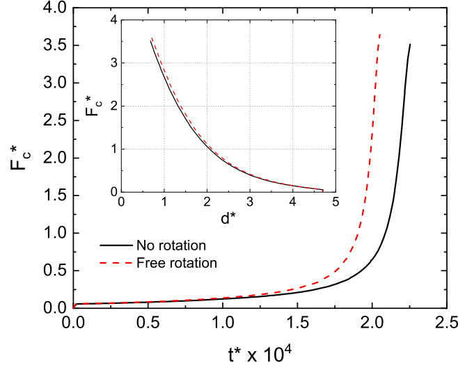
Figure 4: Capillary interaction force ( F_c^* = F_c/(\sigma Bo^2) ) for rotating and non-rotating cylinders as a function of time ( t^* ). Inset: F_c^* versus the center-to-center distance ( d^* = d/L_c ). Parameters: \mu^* = 0.1 , \theta = 100^\circ , Cn = 0.04 , see also table 1.
