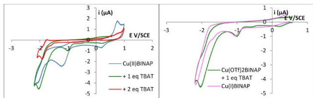
Figure 3. Cyclic Voltammograms in THF + 0.1 M \text{NBu}_4\text{BF}_4 , at a gold disc microelectrode (0.25 mm diameter) at v = 0.5 \text{ V}\cdot\text{s}^{-1} and at r.t. a- 10^{-2} \text{ M Cu(OTf)}_2 + 1 molar equiv. of BINAP (blue curve); b- + 1 molar equiv. TBAT (green curve); c- + 2 molar equiv. TBAT (red curve).
