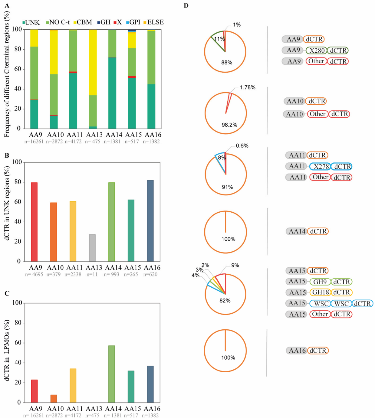
Figure 1. Nature of C-terminal regions occurring in LPMOs. (A) Description and abundance of the various C-terminal regions in LPMO families. LPMOs without any C-terminal region downstream the catalytic domain are denoted as “NO C-t”. The “Else” category includes cell wall retention motifs (for AA10, Pfam PF00746) and barwin domains (for AA15; Pfam PF00967). (B,C) LPMO family-dependent percentage of LPMO-dCTRs among LPMOs with UNK regions (B) and among all LPMO sequences (C). LPMO-dCTRs are LPMOs predicted to have at least one LDR. “n” is the number of sequences analyzed for each LPMO family. (D) Domain architecture of LPMO-dCTRs. Others modules include different CBMs, X domains and combinations of both.
