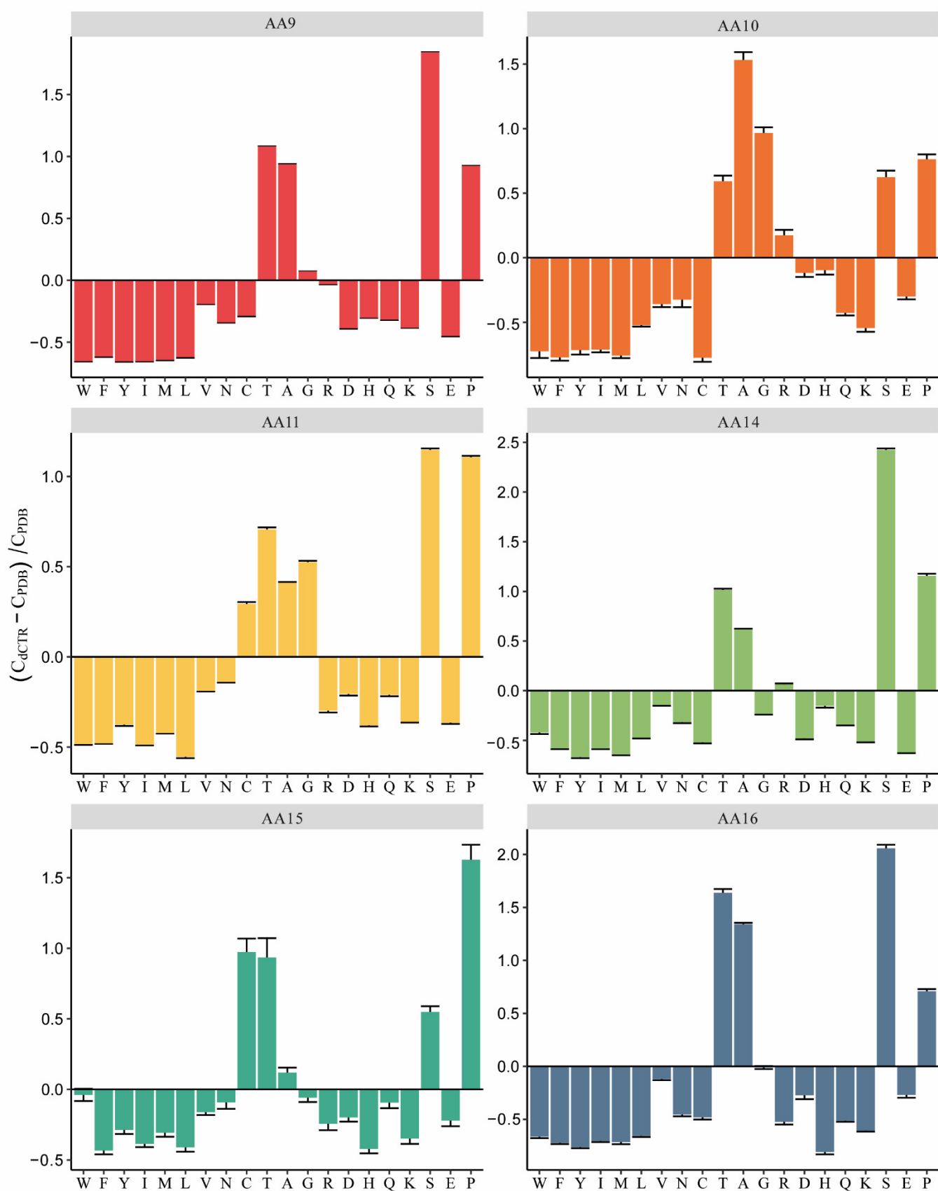
Figure 3. Compositional bias of dCTRs with respect to the PDB database, across the different LPMO families. The fractional difference in the amino acid composition was evaluated as (C_{dCTR} - C_{PDB}) / C_{PDB} , where C_{dCTR} is the content in a given
