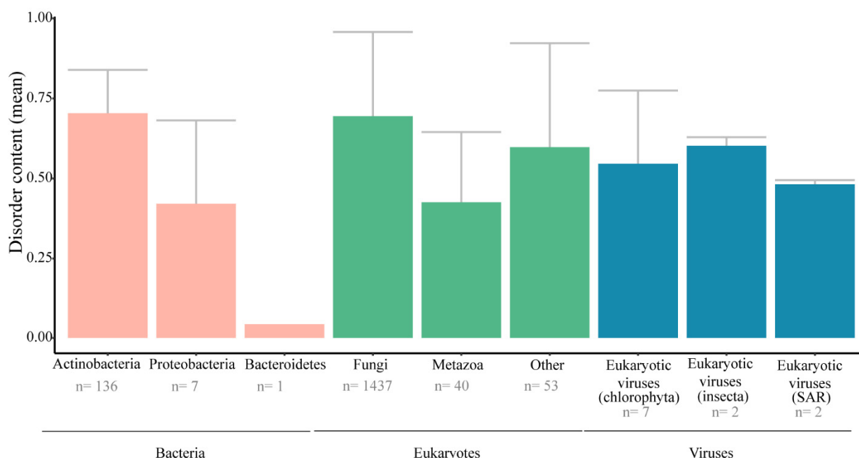
Figure 6. Disorder content of dCTRs in LPMOs across kingdoms. The disorder content is calculated as the mean of the fraction of disordered residues within dCTRs. The eukaryotes category Metazoa includes arthropods and mollusks and the category “Other” includes algae and oomycetes. Abbreviations: SAR, Stramenopiles , Alveolata , Rhizaria ; n is the number of species having LPMO-dCTRs.
