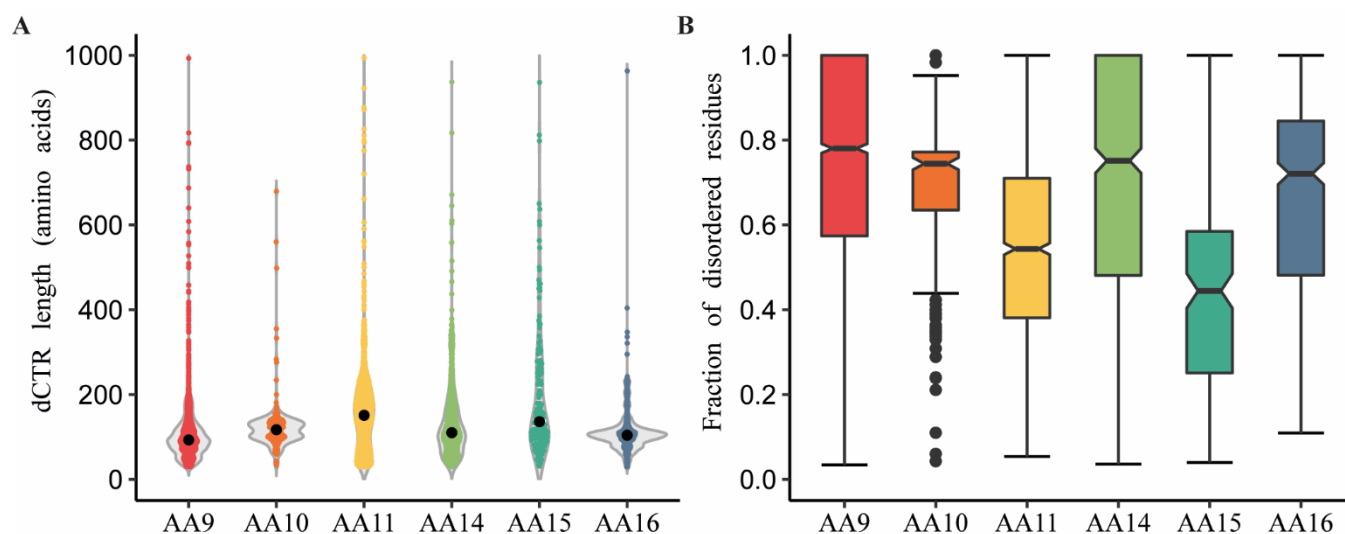
Figure 2. Length and disorder content of the dCTRs. (A) Violin plots showing the distribution of the length of dCTRs across the different LPMO families. The dot in each violin plot represents the median length value. (B) Boxplots showing the fraction of disordered residues within dCTRs across the LPMO families. The central box shows the middle portion (i.e., 25–75%) of the dataset: the bottom line of the box defines the first quartile (25%), the middle line shows the median, and the top line of the box shows the third quartile (75%). The extremities of vertical whiskers represent the largest and smallest values. Outliers are represented by a dot (AA10 family).
