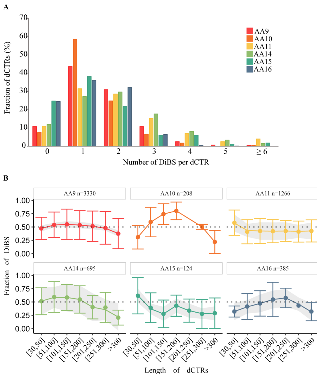
Figure 5. Prediction of Disordered Binding Sites (DiBSs) in dCTRs. (A) Number of DiBS predicted by ANCHOR2 across the LPMO families. (B) Fraction of DiBSs, i.e., number of residues in DiBS divided by the length of dCTRs, plotted as a function of the length of dCTRs across LPMO families, with n being the number of sequences per family having at least one DiBS.
