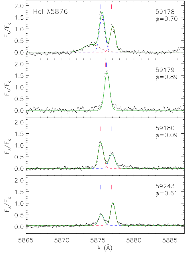
Fig. 7. Residual UVES He I \lambda 5876 Å profiles (black dots). In each panel, the two-Gaussian fit to the emission peaks (green full line) and the individual Gaussians corresponding to the primary (blue dashed line) and secondary (red dashed line) component are overlaid. The blue and red vertical ticks mark the expected position of the lines of primary and secondary component, respectively, according to the photospheric RV. The dashed brown line in the upper panel represents the Gaussian fitted to the excess blueshifted emission observed only in this spectrum. The reduced Julian day and the orbital phase ( \phi ) are marked in the upper right corner of each box.
