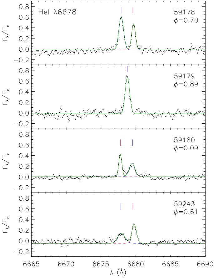
Fig. 6. Residual UVES spectra in the He I \lambda 6678 Å region (black dots). In each panel, the two-Gaussian fit to the emission peaks (green full line) and the individual Gaussians corresponding to the primary (blue dashed line) and secondary (red dashed line) component are overlaid. The blue and red vertical ticks mark the expected position of the lines of primary and secondary component, respectively, according to the photospheric RV. The reduced Julian day and the orbital phase ( \phi ) are marked in the upper right corner of each box.
