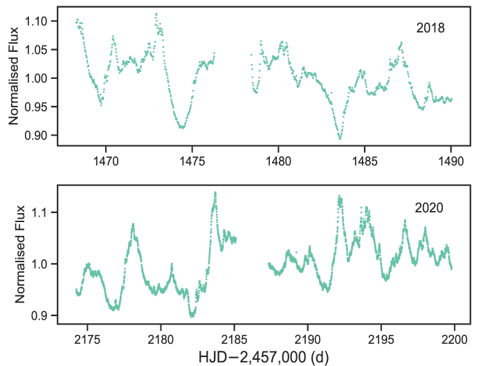
Fig. 1. TESS light curves of CVSO 104 A+B in 2018 (top) and 2020 (bottom).
