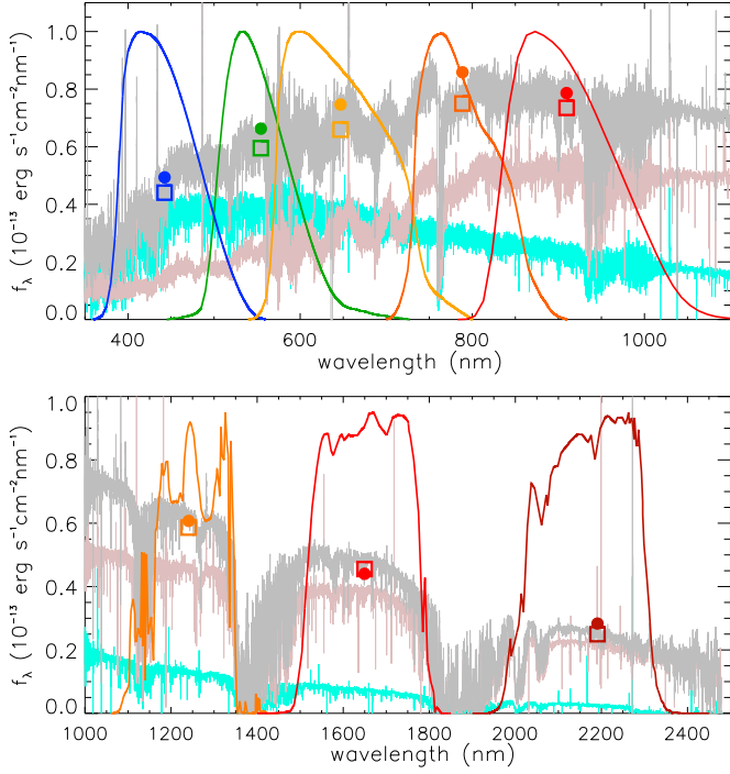
Fig. 10. X-Shooter flux-calibrated spectrum of CVSO 104 A (pink line), CVSO 104 B (cyan line), and the sum of the two (grey line) in the visual ( top panel ) and NIR region ( bottom panel ). The contemporaneous photometry obtained from OACT in the BVR_C I_C z' bands and the 2MASS JHK_s photometry are displayed with colored dots. The filter bandpasses and the synthetic photometry (open squares) obtained integrating the combined spectrum (A+B) over these bandpasses are overlaid with the same color as the photometric points.
