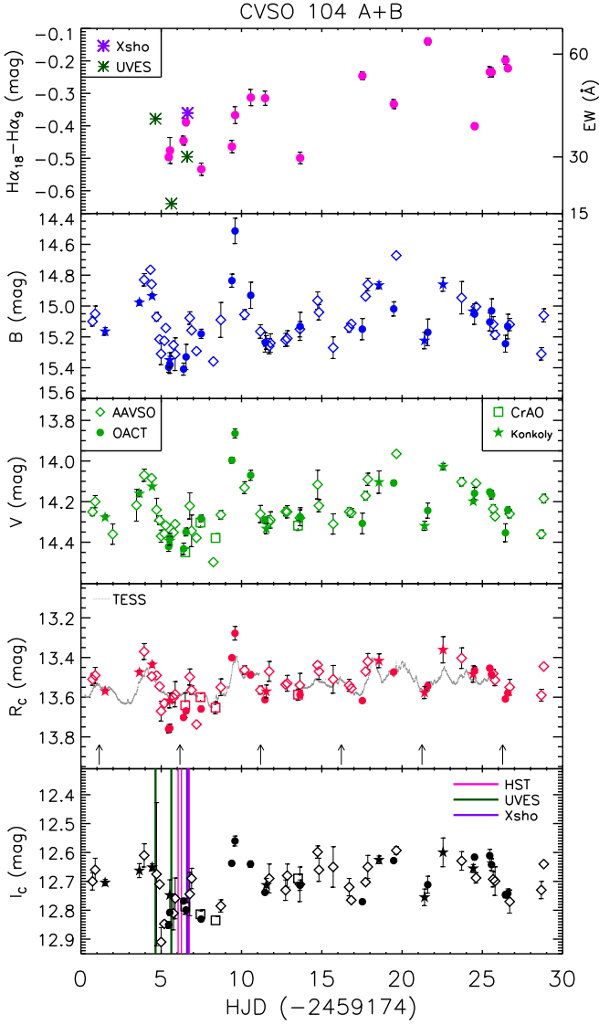
Fig. A.1. Multiband ground-based light curve of CVSO 104A+B around the time of VLT and HST observations. Different symbols, as reported in the legend, are used for the different data sets. The H\alpha color index, which measures the intensity of the line, is shown in the upper panel. Synthetic H\alpha colors based on X-Shooter and UVES spectra are overplotted with asterisks in the same box. The contemporaneous TESS light curve is overplotted with grey dots to the R_C light curve. The arrows in the same box mark the periastron passages. The epoch of VLT and HST observations are marked in the lower box.
