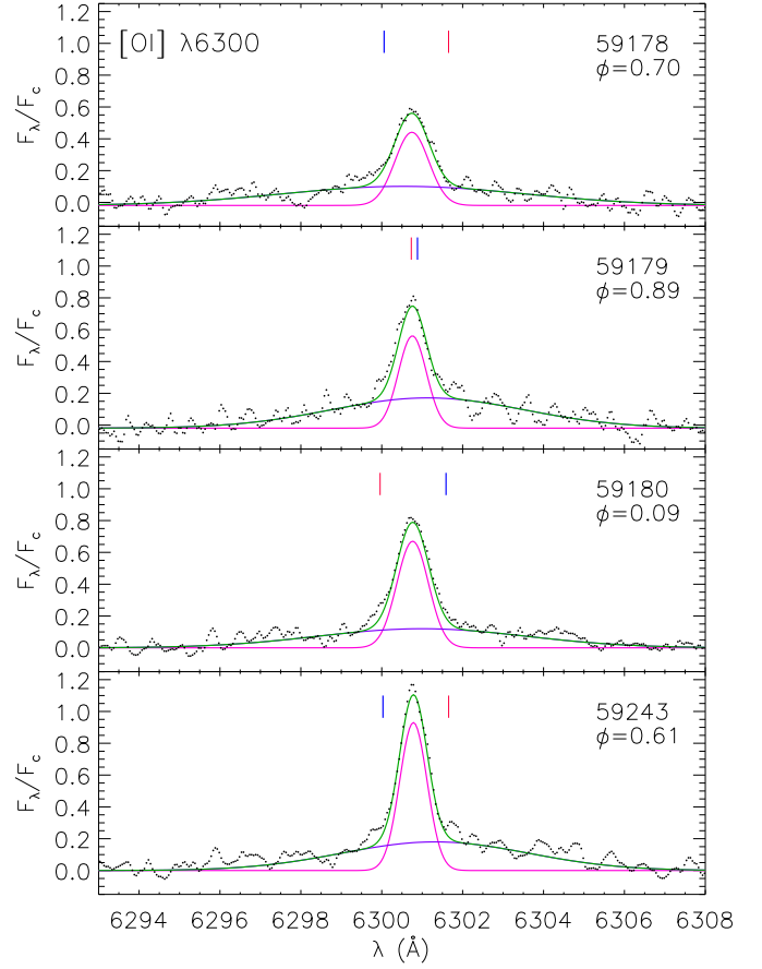
Fig. 9. Residual UVES spectra in the [O\ I] \lambda 6300 region (black dots). The blue and red vertical ticks mark the expected position of the lines of primary and secondary component, respectively, according to the photospheric RV. The Gaussian fits to the broad and narrow component of the line profile are overplotted with purple and magenta lines, respectively, while their sum is plotted with a green line. The reduced Julian day and the orbital phase ( \phi ) are marked in the upper right corner of each box.
