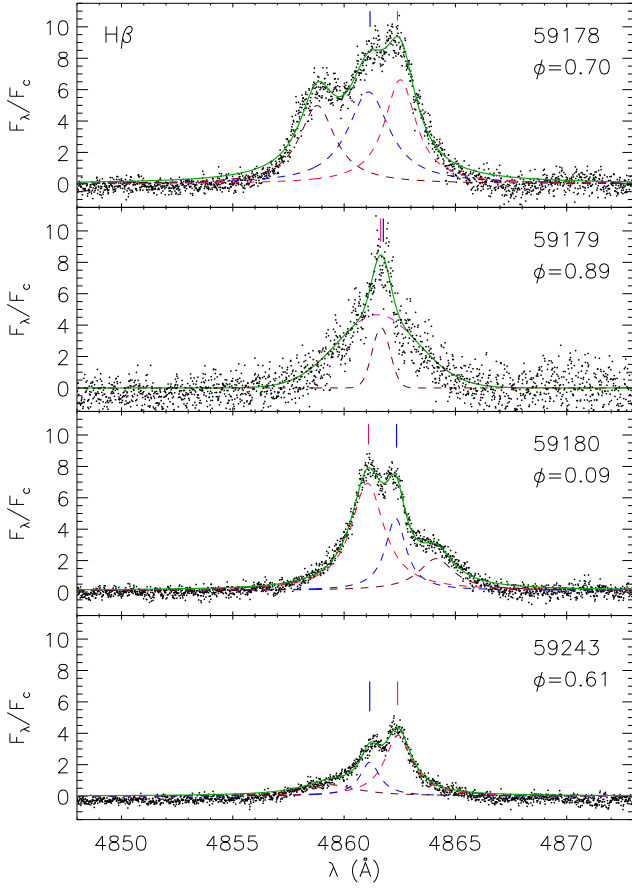
Fig. 8. Residual UVES H\beta profiles (black dots). The meaning of the symbols is as in Fig. 7.
