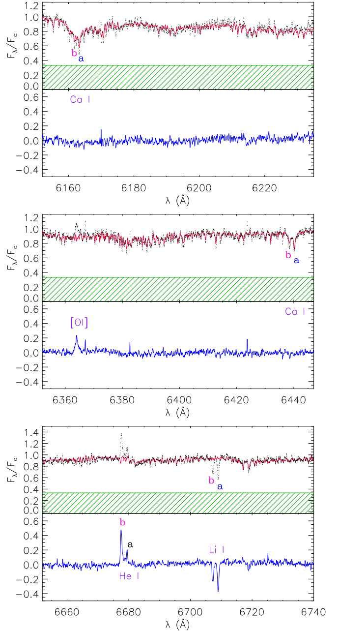
Fig. 4. UVES spectrum of CVSO 104 A (black dots) observed on JD = 2 459 180 in three spectral regions around 6200 Å (top), 6400 Å (middle), and 6700 Å (bottom). In each box the synthetic spectrum, which is the weighted sum of two standard star spectra mimicking the primary and secondary component, is overplotted with a full red line. Prominent lines from the primary and secondary component are marked with a and b, respectively. The hatched green regions denote the level of the veiling. The residual spectra obtained by the subtraction of the photospheric template are displayed in the lower panel of each box with a blue line.
