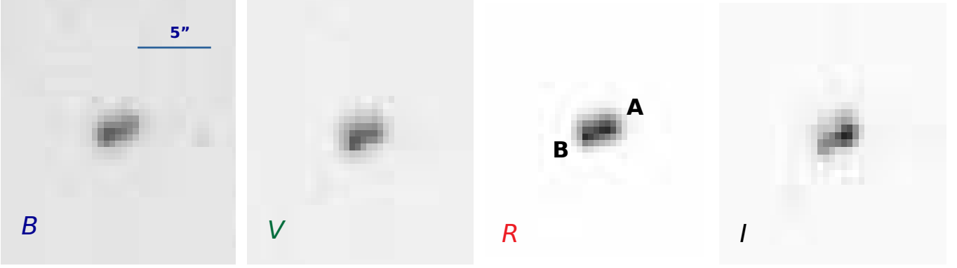
Fig. 2. Portion of images acquired at OACT on 16 Dec 2020 in BVRI bands centered on the visual pair CVSO 104 A+B. North is up and East to the left and the two components are indicated in the R -band image. Note how the relative brightness of the two stars changes in the different bands, with A becoming brighter than B in the I band.
