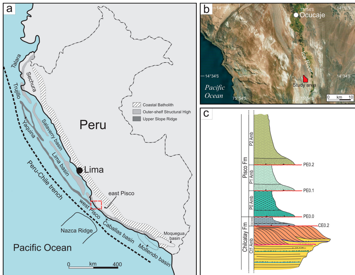
Figure 1. (a) Map of the major structural trends and basins of coastal Peru, redrawn and modified from Travis, Gonzales, and Pardo (1976) and Thornburg and Culm (1981). The red dashed rectangle outlines location of the area shown in detail in Figure 1(b); (b) close up of the red dashed inset box in Figure 1(a) showing the geographic location of the study area along the western side of the Ica River valley; (c) Schematic stratigraphic column with the main subdivisions and units (not to scale).
