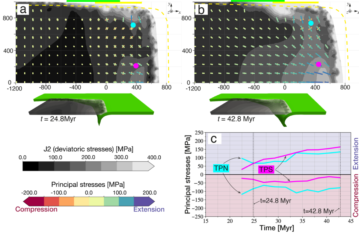
Figure 6: a-b) Snapshots of the time-evolution of the model performed with R=200 km and with a weaker overriding plate ( 3 \times 10^{23} Pa s) than the reference model. The dashed yellow lines display the shape of the overriding plate in the reference model at equivalent stages of subduction (different times but with the same depth reached by the southernmost slab tip). See Figure 4 for other legend details.
