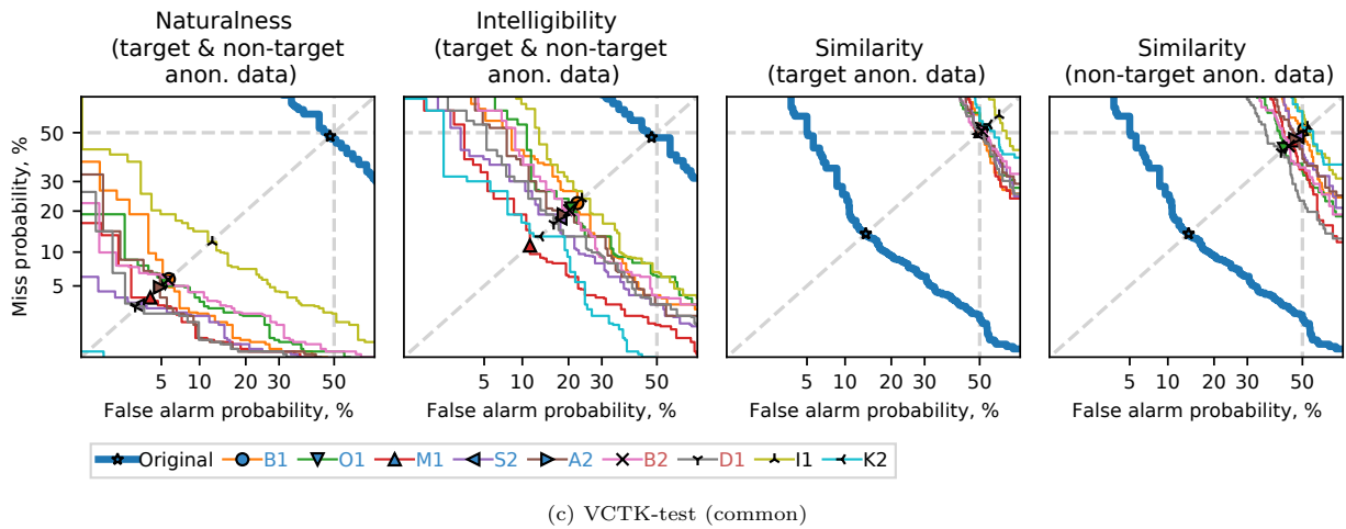
Figure 26: DET curves for each test set.
