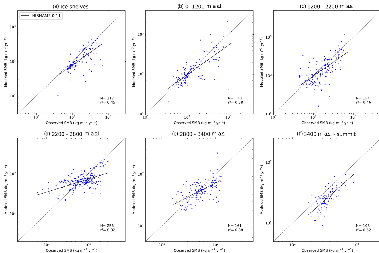
Figure A4. Comparison between HIRHAM5 0.11° and observed SMB (units: kg m -2 yr -1 ) over the ice shelves (a) and by elevation classes (b–f). Due to the use of logarithmic axes, only positive values for the observed and modelled SMB from all the RCMs in this study are used (number for each bin N ). Finally, the regression coefficient of each regression line is also shown ( r^2 ).
