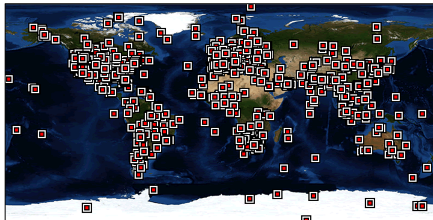
Figure 2. Location of sun/sky photometers belonging to the AERONET network (red dots), courtesy of https://aeronet.gsfc.nasa.gov (last consulted on 4 August 2021).
