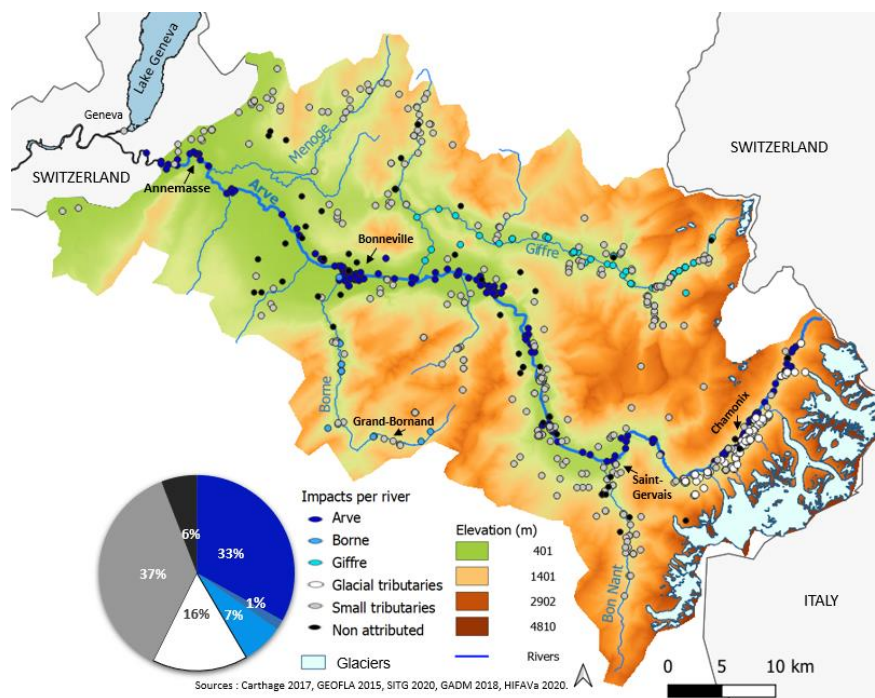
Figure 4. Location and distribution of flood impacts caused by the Arve and its tributaries. The category “non attributed” corresponds to the part of impacts for which it was not possible to attribute a river, either because events are related to overland flows or because of the location between two or more rivers.
