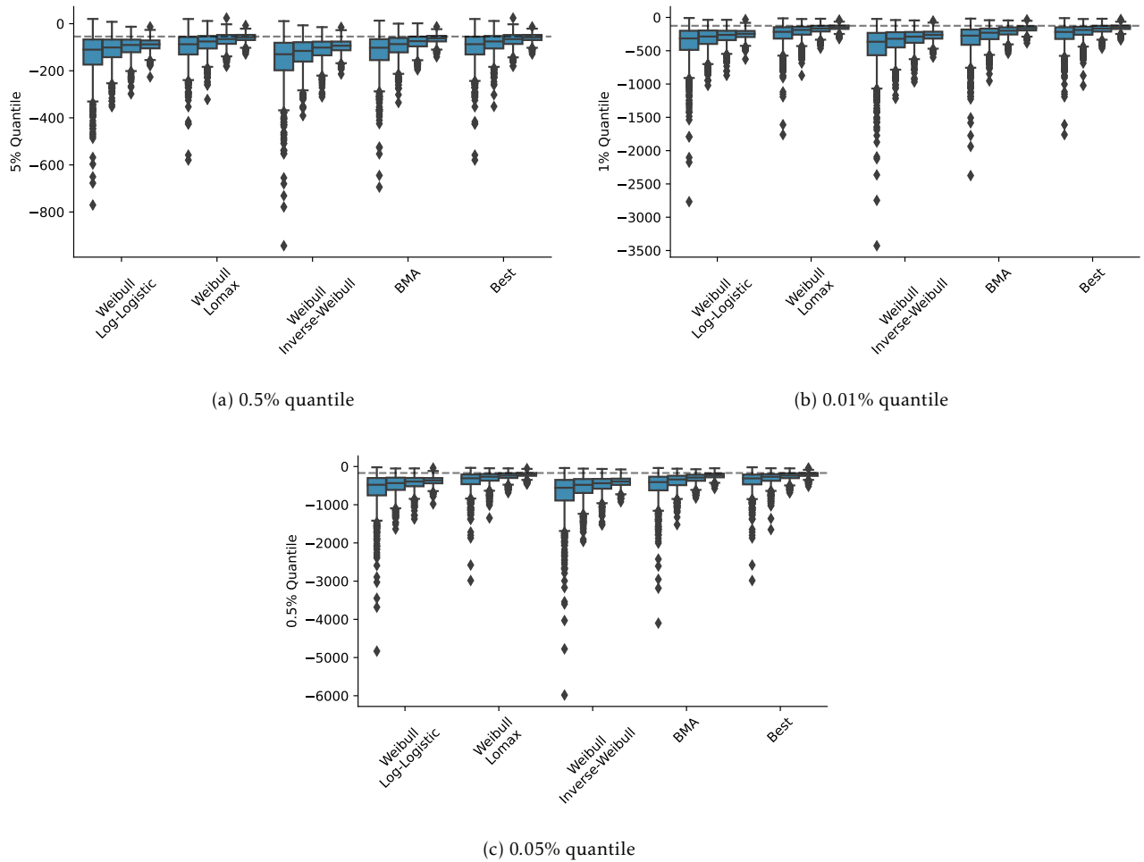
Figure 2: Left quantiles of the profit and loss distribution of the first-line insurer depending on the composite model used. The loss data consists of sample of sizes 500, 1000, 2000, and 5000 drawn from a continuous Weibull – Lomax composite model. The dashed line represents the true value.
