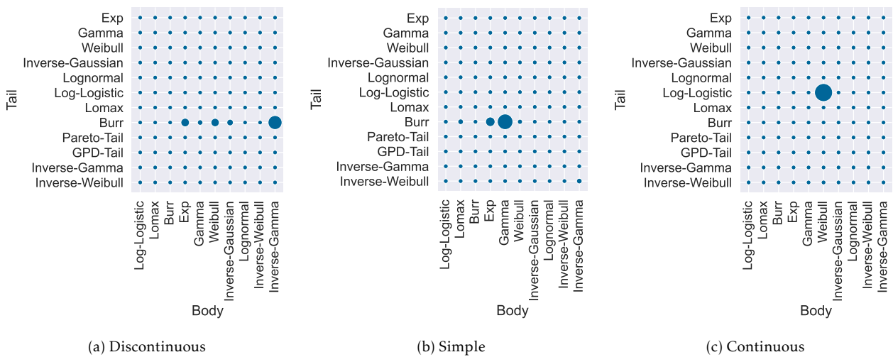
Figure 6: Posterior probabilities of the composite models depending on their type.
