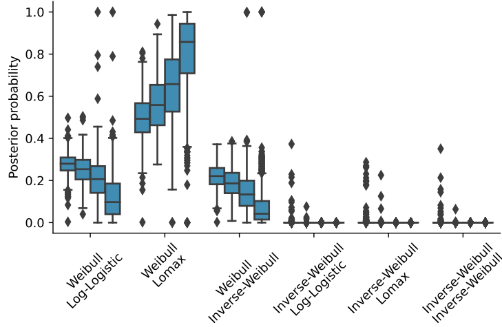
Figure 1: Posterior probabilities assigned to each composite model for sample of sizes 500, 1000, 2000, and 5000 drawn from a continuous Weibull – Lomax composite model.
