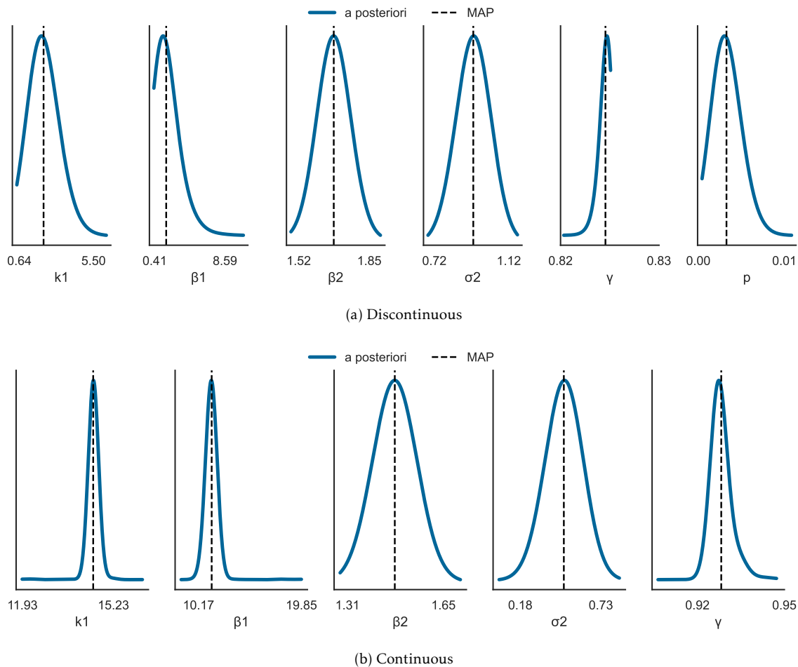
Figure 8: Posterior plots of the composite model parameters.
