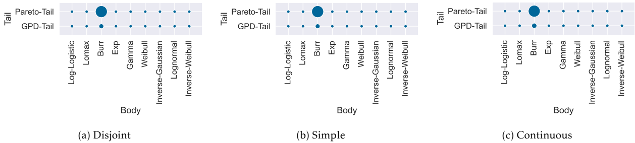
Figure 10: Posterior probabilities of the composite models depending on their type with the fixed threshold.
