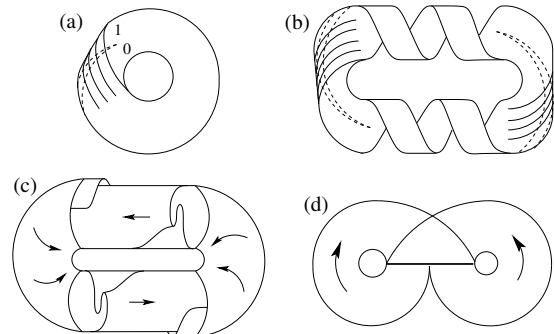
FIG. 14. Branched manifolds describing (a) Rössler, (b) periodically driven Duffing, (c) van der Pol attractors, and (d) Lorenz attractors for particular parameter values. Redrawn from The topology of chaos , p. 133, (Wiley, 2003).
