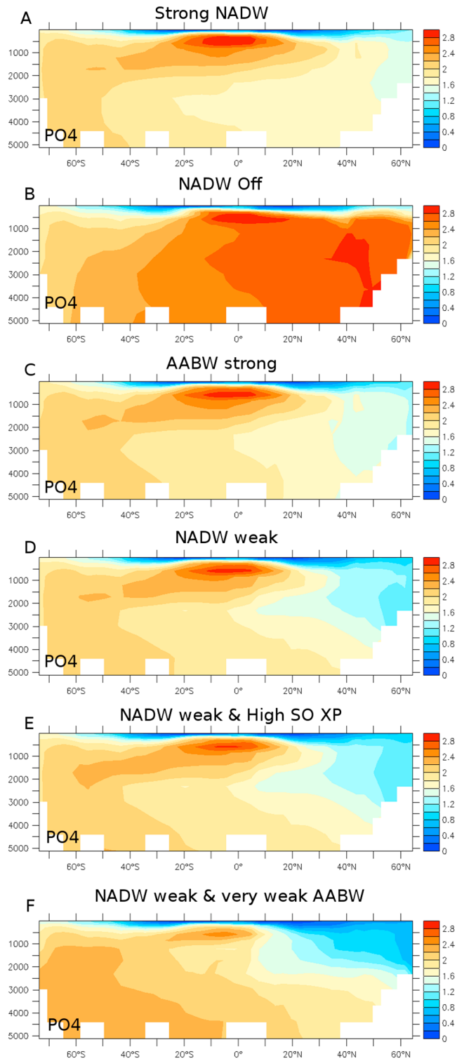
Figure 3. Phosphate content ( \mu\text{mol/L} ) zonally averaged over the Atlantic for LGM simulations with (a) strong NADW (V3L*), (b) NADW Off (V3LNAoff+), (c) strong AABW (V3LNAwSOs \Delta ) (d) weak NADW (V3LNAw \bullet ), (e) weak NADW and enhanced Southern Ocean export production (V3LNAwGR \circ ), and (f) weak NADW and very weak AABW obtained through both buoyancy forcing and 20% reduced Southern Hemispheric westerlies (V3LNAwSOwSHWw \star ).
