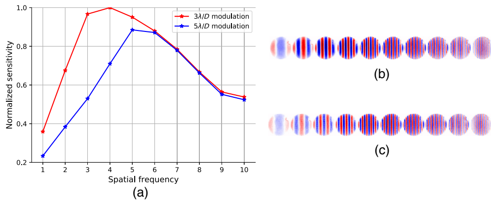
Fig. 8 Response of the Keck PyWFS to different spatial frequencies: (a) measured sensitivity for 3\lambda/D and 5\lambda/D modulation, example PyWFS signals for (b) 3\lambda/D modulation, and (c) 5\lambda/D modulation.
