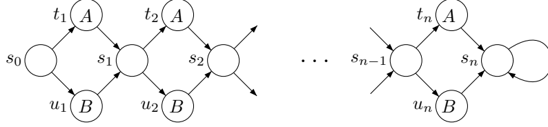
FIG. 3. The structure T_n
