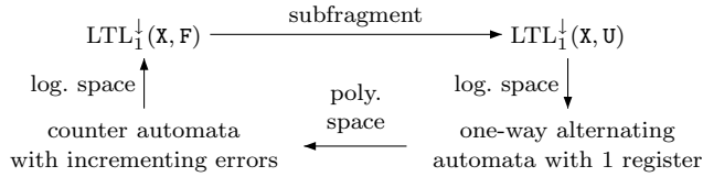
Fig. 1. A circle of translations which preserve language nonemptiness
