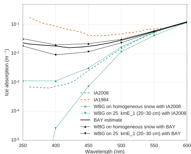
Figure 16. Ice absorption estimated with the WBG method applied to simulated irradiance profiles with MCML in the presence of the rod for the homogeneous snowpack (triangles up) and the 25kmE_1 snow pit (triangles down) by using IA2008 (green) and BAY (black) ice absorption spectra, respectively, as input.
