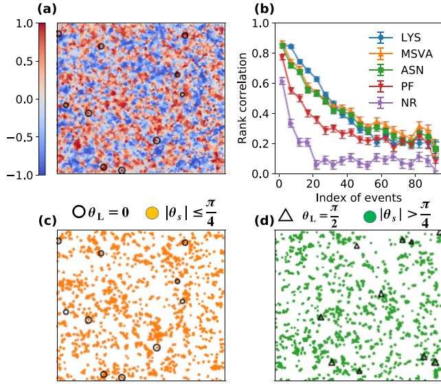
FIG. 2. Predicting plastic events by analyzing initial configurations. (a) The correlation field of atomic shear nonaffinity \hat{G}(\theta_L = 0) and the locations of the first ten plastic events (black circles) triggered in shear protocols with \theta_L = 0 . (b) Correlation between the indicators including local yield stress (LYS), mean-square vibrational amplitude (MSVA), atomic shear nonaffinity (ASN), participation fraction (PF), and nonaffine rate (NR) with the locations of plastic events as a function of the index of the events. Averages are taken over windows of five events. The error bar at each window represents the standard deviation of the mean. (c) Orange circles represent the atoms with RC_{\hat{G}} > 0 and |\theta_s| < \frac{\pi}{4} . Black circles mark the locations of the first ten plastic events with \theta_L = 0 . (d) Green circles represent the atoms with RC_{\hat{G}} > 0 and |\theta_s| > \frac{\pi}{4} . Triangles mark the locations of the first ten plastic events with \theta_L = \frac{\pi}{2} .
