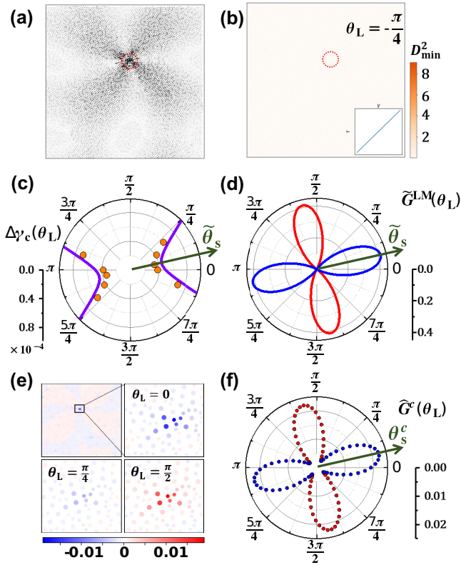
FIG. 1. Analysis of configuration that was sheared to be close to the triggering of a plastic event. (a) The spatial distribution of the normal mode with lowest eigenvalue. (b) The D_{\min}^2 field [26] after shear with strain of \Delta\gamma = 6 \times 10^{-5} in the orientation of \theta_L = -\pi/4 . The inset shows the stress-strain curve. (c) The predicted triggering strain (line) and triggering strain from simulation (circles) as a function of shear angle \theta_L . (d) The magnitude of nonaffine modulus contribution from the lowest mode at different \theta_L . The blue line represents the range of \theta_L , where the plastic event can be triggered, while the red line represents the range of \theta_L , where the plastic event cannot be triggered. (e) The spatial distribution of \hat{G}(\theta_L)\text{sign}(\Delta\gamma_c(\theta_L)) for different orientations. (f) The atomic shear nonaffinity in different orientations for the atom that has the maximum magnitude of atomic shear nonaffinity in (e).
