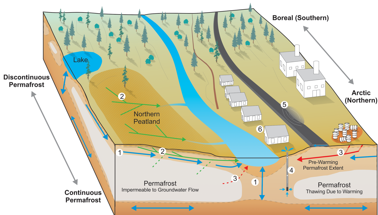
Figure 1. Pathways for groundwater to catalyse environmental change in the Arctic. (1) Arctic warming and permafrost thaw promote increased flux, circulation, and connectivity of groundwater above and below permafrost. (2) Groundwater transports carbon and nutrients from terrestrial to aquatic environments via progressively deeper subsurface flow paths with top-down permafrost thaw (green arrows). Permafrost carbon may be mobilized in the aqueous phase upon thaw and transported to inland waters (dashed green lines and arrows). (3) As permafrost thaws, there are opportunities for increased transport of contaminants (e.g. industrial waste, sewage) due to enhanced groundwater flow (red arrows). Sequestered contaminants, such as pathogens or mercury, are released as permafrost thaws and transported via groundwater flow (dashed red arrow). (4) Water resources will change as permafrost thaws, including increased potential for groundwater development. (5) Groundwater flow can enhance permafrost thaw rates, leading to land subsidence and destruction of surface infrastructure such as roads or buildings. (6) The incorporation of cryohydrogeology in planning for northern communities and future economic development would enhance resiliency in the face of environmental changes.
