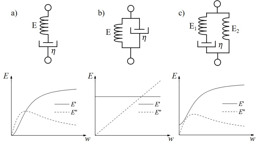
Figure 6: a) Maxwell, b) Voigt and c) the standard linear solid simplified elastic-viscous models are depicted in analogy with equivalent electrical circuits. Young's modulus E is analogous to a real-valued admittance, whereas viscosity contributes a i\omega\eta admittance similar to a capacitance. The resulting relationship between dynamic modulus and angular frequency is depicted below each equivalent circuit model (see text for their expressions).
