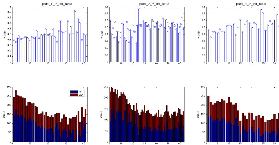
FIGURE 4. Georgian paki \rightarrow paik . Top panels: ratio vocalic portion to inter-burst interval (IBI). Bottom panels: vocalic portion duration in red (ms) overlaid on IBI duration in blue (ms).
