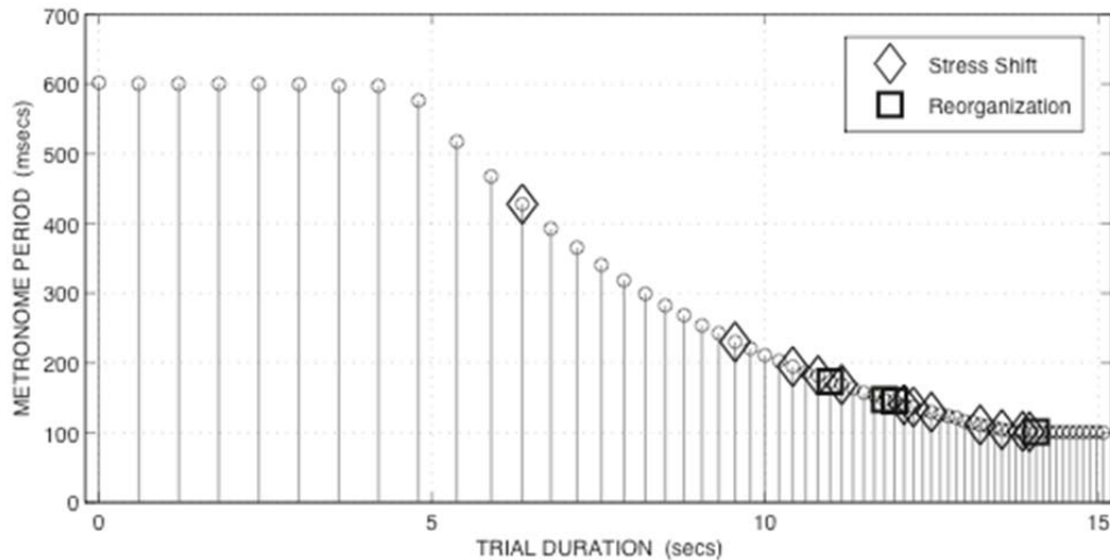
FIGURE 2. CCV reorganization: results for p^h a t^h a pooled across all trials and speakers (some transition points contain multiple events). All nine speakers shifted stress ( páta \rightarrow patá ). Seven speakers also showed initial vowel elision ( patá \rightarrow ptá ).
