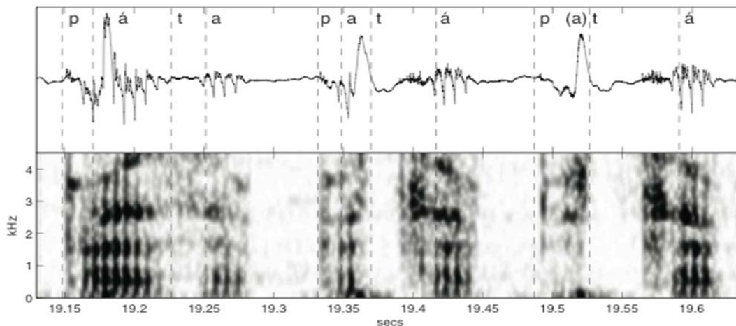
FIGURE 1. Georgian. Example shift from initial to final prominence in [p h at h a] (V2 duration increases relative to V1), followed by elision of V1 ( pata → pta ). Speakers typically persist in the CCV pattern following reorganization.
