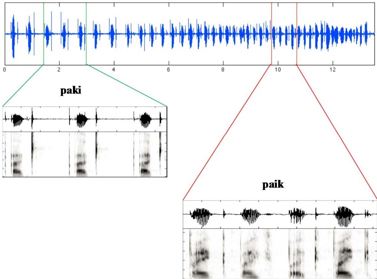
FIGURE 3. Georgian paki \rightarrow paik . Re-phasing of /k/, as rate increases.
