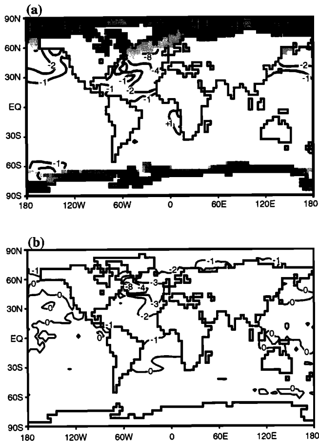
Figure 1. Differences of the boundary conditions between the control and cold climate experiments: (a) mean anomalies of sea surface temperatures (SSTs) and sea ice (temperature contour lines at -1^{\circ}\text{C} , -2^{\circ}\text{C} , -4^{\circ}\text{C} , -8^{\circ}\text{C} , and -16^{\circ}\text{C} ; heavily shaded area: sea ice prescribed in both climates at least half of the year, lightly shaded area: additional sea ice prescribed at least half of the year for the cold climate), (b) anomalies of isotope composition of the ocean surface water \delta^{18}\text{O}_{\text{ocean}} (contour lines at 0\text{‰} , -1\text{‰} , -2\text{‰} , -3\text{‰} , -4\text{‰} , and -8\text{‰} ).
