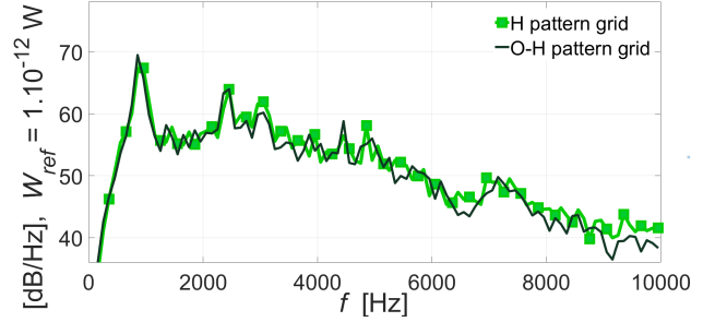
Figure 18: Downstream sound power per vane of a 3 channels computation (baseline geometry) for the H and O-H pattern meshes. Averaging over 100 Hz bands.
