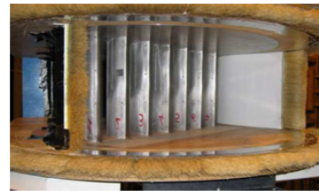
Figure 1: Picture of the rectilinear cascade facility [1].
