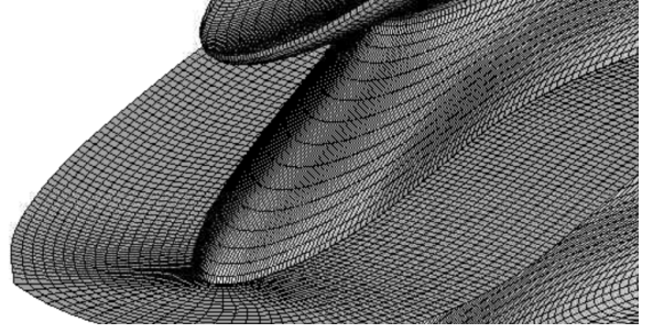
Figure 17: Zoom on slices of the serrated mesh extruded from a O-H patterned grid.
