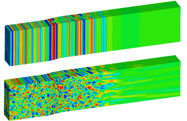
Figure 6: Snapshots of u'_y [ \text{m}\cdot\text{s}^{-1} ] for the parallel (top) and oblique (bottom) gusts (levels between -2 and 2).
