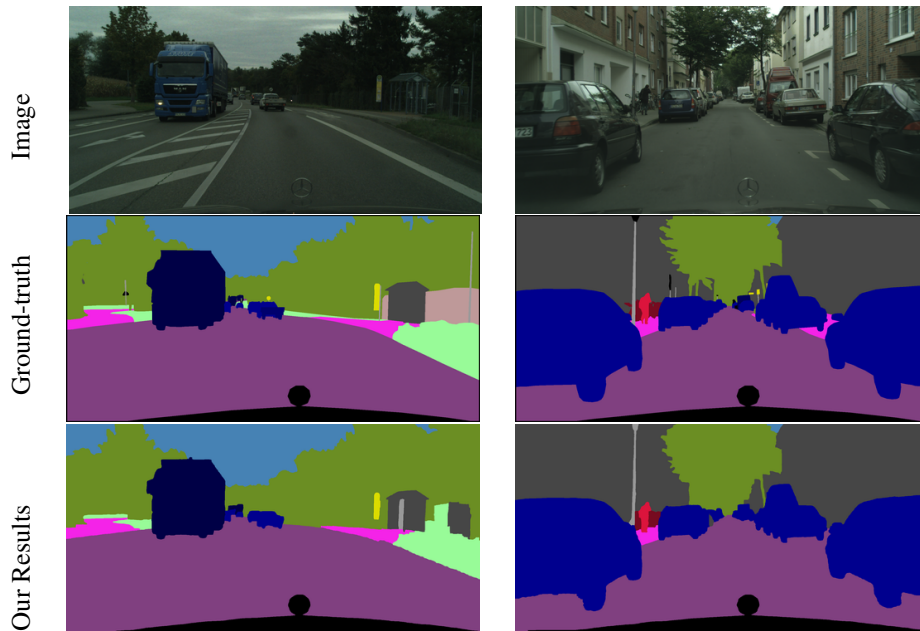
Figure 9: Cityscapes result, each column is a different image, row indicates which kind.
