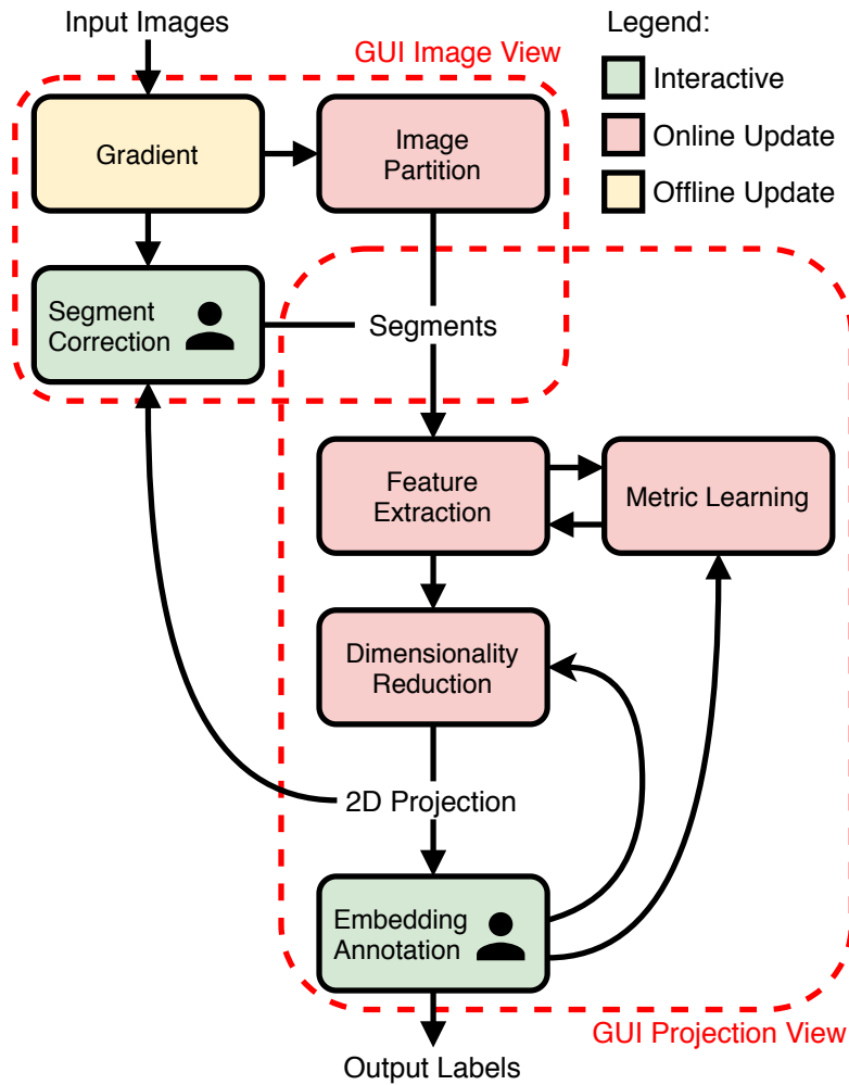
Figure 2: The proposed feature space annotation pipeline.
