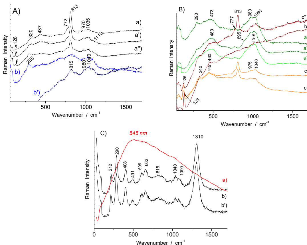
Figure 13. Representative Raman spectra recorded on the painted enamels of the F1341C bottle: (A) white (a,a',a'') and blue (b,b'); (B) green (a,a',a'' light green) and yellow (b,c,c',c''); (C) orange (a) and red (b,b').
