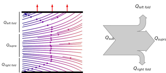
Fig. 1: Example of the velocity field during the glottal opening (on left) and representation of the volume flow division (on right).
