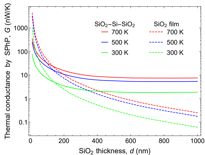
Figure 5. A comparison of the SPhPs thermal conductances of the SiO 2 /Si (10 \mu m)/SiO 2 three-layer structure and of a single SiO 2 film at 300, 500 and 700 K, for different SiO 2 thicknesses.
