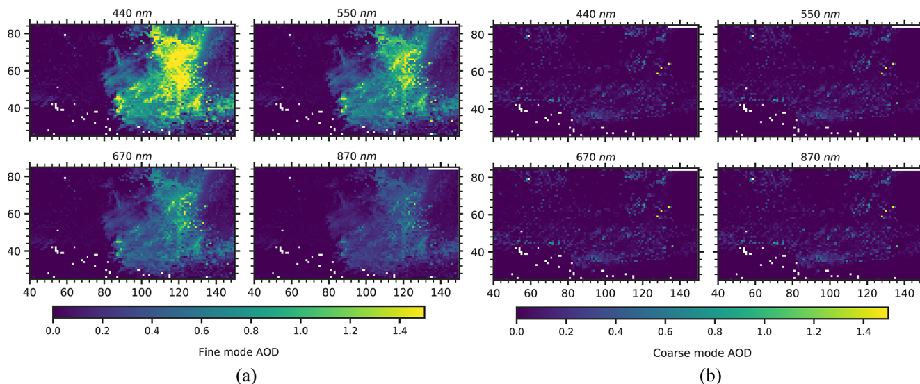
Figure 10. (a) Fine-mode AOD map of a subsetted portion of the 27 October 2017 T18:16 UTC smoke scene that was marked by a red rectangular box in Fig. 8 for all AirHARP spectral bands; (b) same as (a) but for coarse-mode AOD. X and Y axes are the pixel coordinates.
