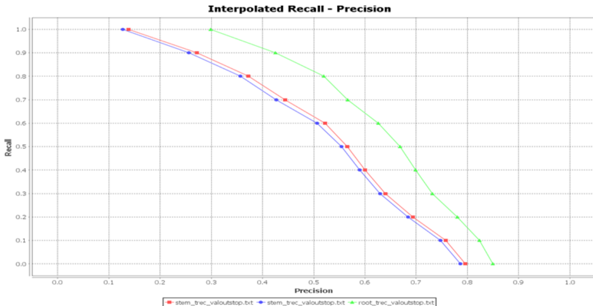
Figure 3: Recall-Precision curves based on stems and roots.
