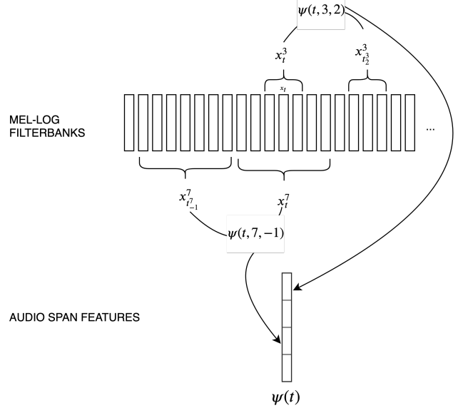
Figure 3: Audio Span Features: It is the concatenation of similarities between the current representation with the 2 \cdot N closest neighbours filterbank representations at different scales s .
