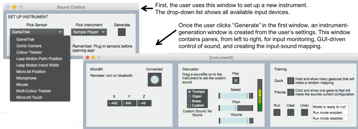
Figure 1: The Sound Control software
