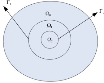
Fig. 1. The domain \Omega = \Omega_0 \cup \Omega_1 \cup \Gamma_1 \cup \Gamma_2 \cup \Omega_2 .
