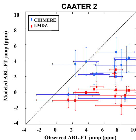
Fig. 6. Comparison of the modelled ABL-FT jumps from LMDZ-ORCHIDEE and CHIMERE-ORCHIDEE to the observed jumps for CAATER 2. Points represent the mean jump for each profile and bars represent the associated \pm 1-\sigma standard deviation from observations and models.
